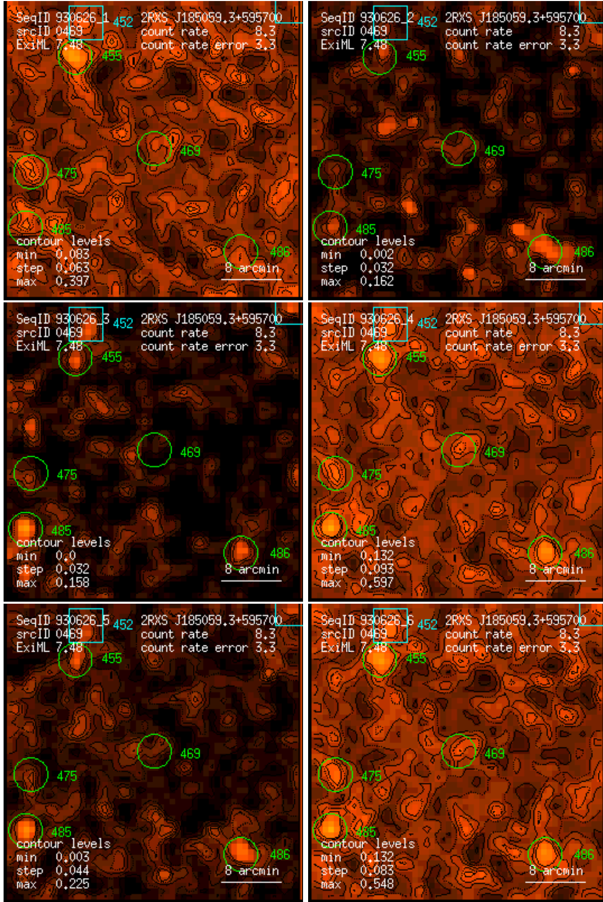
Figure 469: RASS 930626: detection 0469: band rate images, Gaussian filter: (1) PSPC channels 11 – 41, (2) 52 – 90, (3) 91 – 201, (4) 11 – 235, (5) 52 – 201, (6) 11 – 201. Broad band rates in counts/ks. Band rate contour levels in counts/ks/arcmin 2 .
