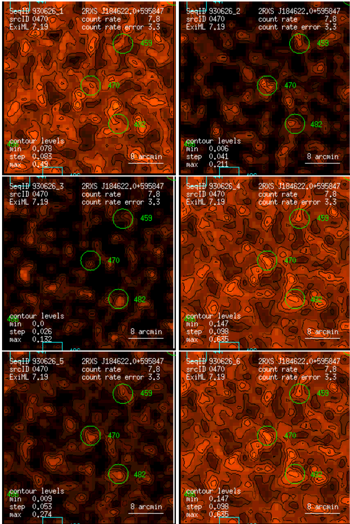
Figure 470: RASS 930626: detection 0470: band rate images, Gaussian filter: (1) PSPC channels 11 – 41, (2) 52 – 90, (3) 91 – 201, (4) 11 – 235, (5) 52 – 201, (6) 11 – 201. Broad band rates in counts/ks. Band rate contour levels in counts/ks/arcmin 2 .
