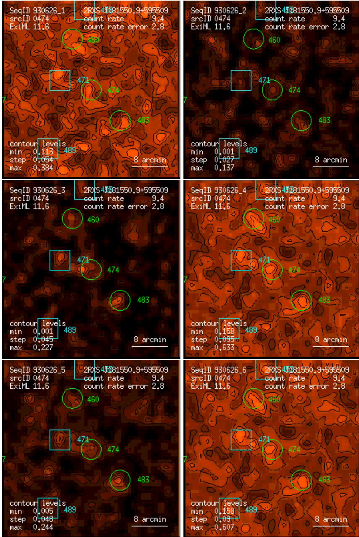
Figure 474: RASS 930626: detection 0474: band rate images, Gaussian filter: (1) PSPC channels 11 – 41, (2) 52 – 90, (3) 91 – 201, (4) 11 – 235, (5) 52 – 201, (6) 11 – 201. Broad band rates in counts/ks. Band rate contour levels in counts/ks/arcmin 2 .
