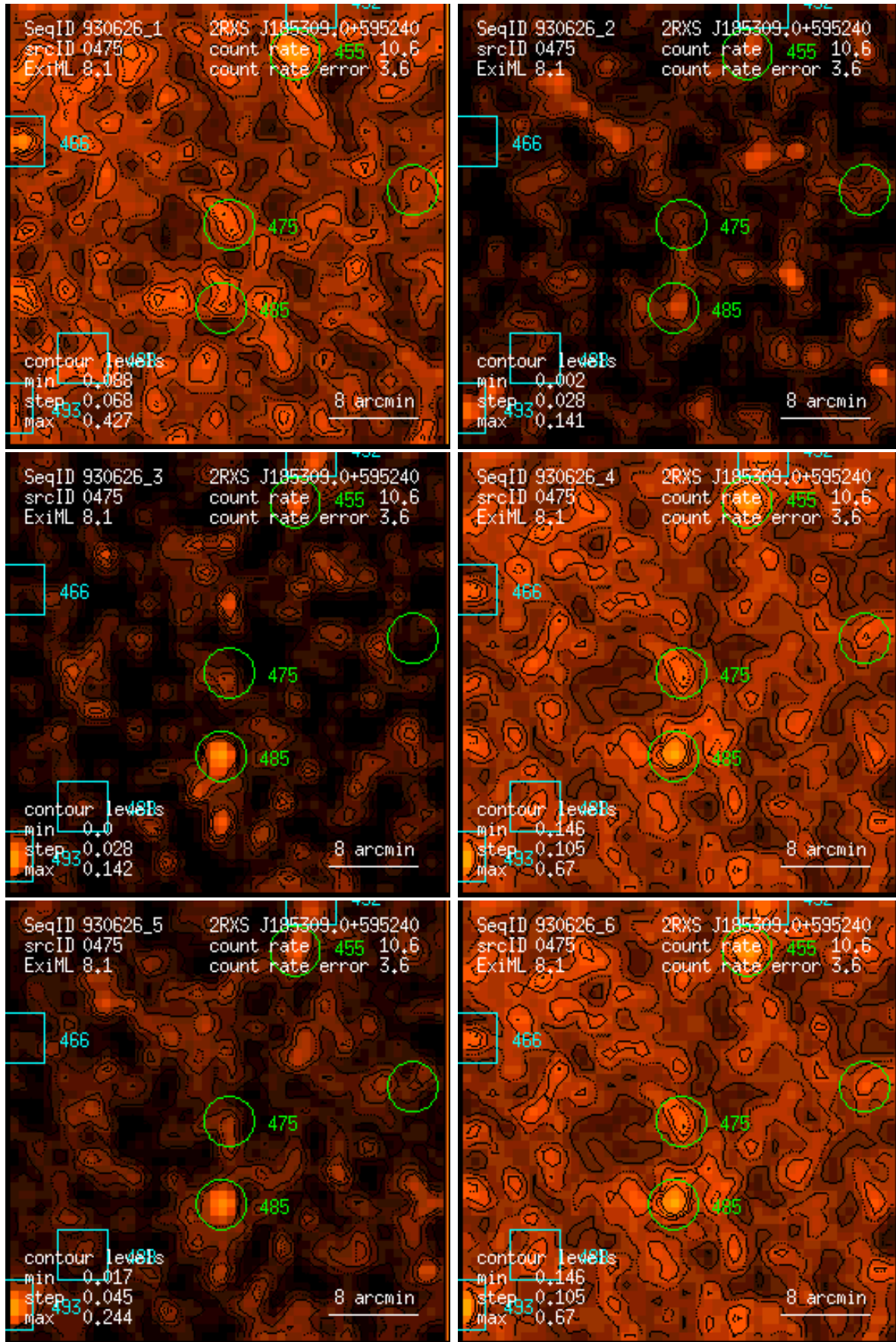
Figure 475: RASS 930626: detection 0475: band rate images, Gaussian filter: (1) PSPC channels 11 – 41, (2) 52 – 90, (3) 91 – 201, (4) 11 – 235, (5) 52 – 201, (6) 11 – 201. Broad band rates in counts/ks. Band rate contour levels in counts/ks/arcmin 2 .
