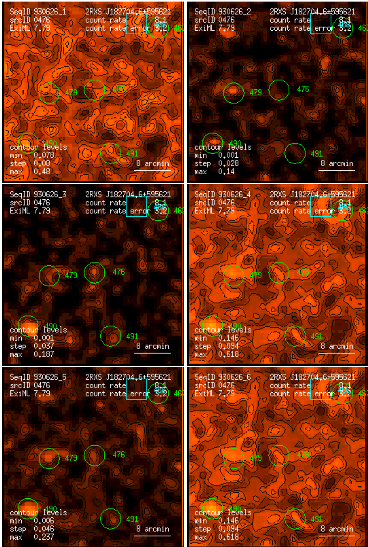
Figure 476: RASS 930626: detection 0476: band rate images, Gaussian filter: (1) PSPC channels 11 – 41, (2) 52 – 90, (3) 91 – 201, (4) 11 – 235, (5) 52 – 201, (6) 11 – 201. Broad band rates in counts/ks. Band rate contour levels in counts/ks/arcmin 2 .
