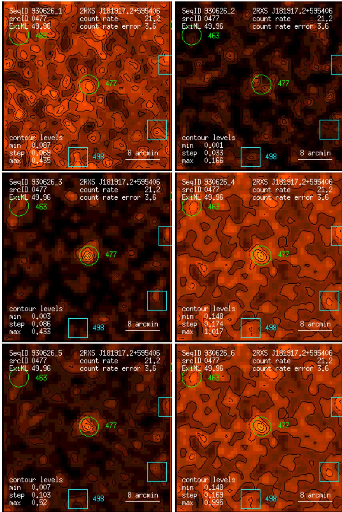
Figure 477: RASS 930626: detection 0477: band rate images, Gaussian filter: (1) PSPC channels 11 – 41, (2) 52 – 90, (3) 91 – 201, (4) 11 – 235, (5) 52 – 201, (6) 11 – 201. Broad band rates in counts/ks. Band rate contour levels in counts/ks/arcmin 2 .
