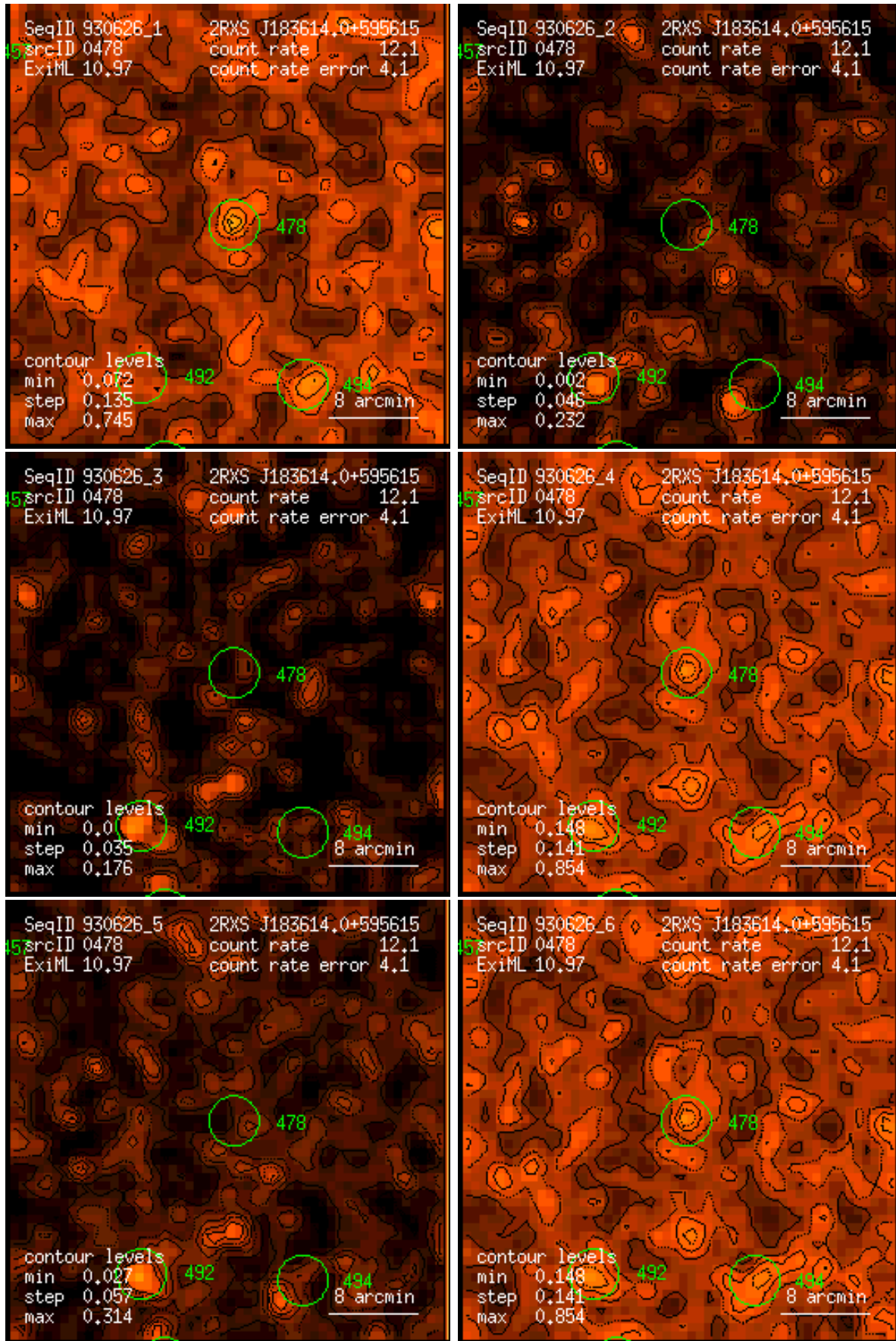
Figure 478: RASS 930626: detection 0478: band rate images, Gaussian filter: (1) PSPC channels 11 – 41, (2) 52 – 90, (3) 91 – 201, (4) 11 – 235, (5) 52 – 201, (6) 11 – 201. Broad band rates in counts/ks. Band rate contour levels in counts/ks/arcmin 2 .
