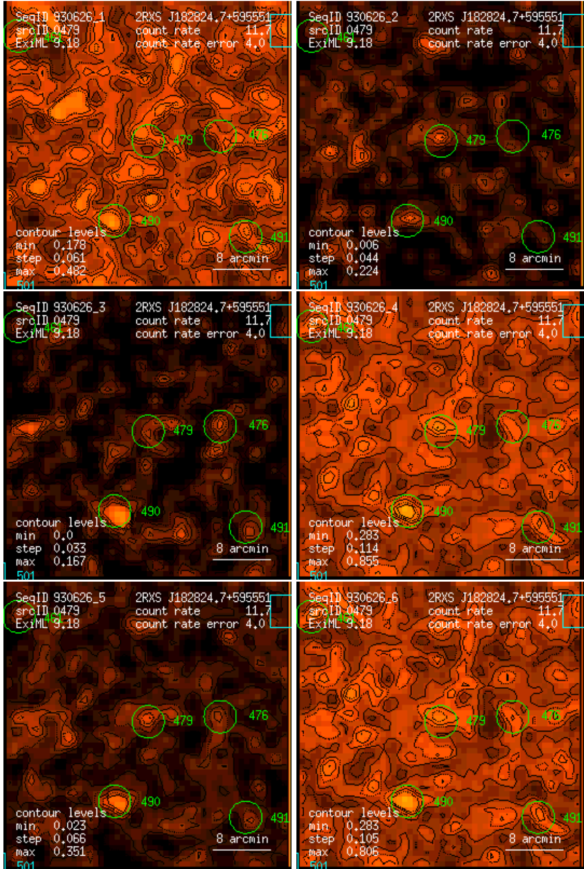
Figure 479: RASS 930626: detection 0479: band rate images, Gaussian filter: (1) PSPC channels 11 – 41, (2) 52 – 90, (3) 91 – 201, (4) 11 – 235, (5) 52 – 201, (6) 11 – 201. Broad band rates in counts/ks. Band rate contour levels in counts/ks/arcmin 2 .
