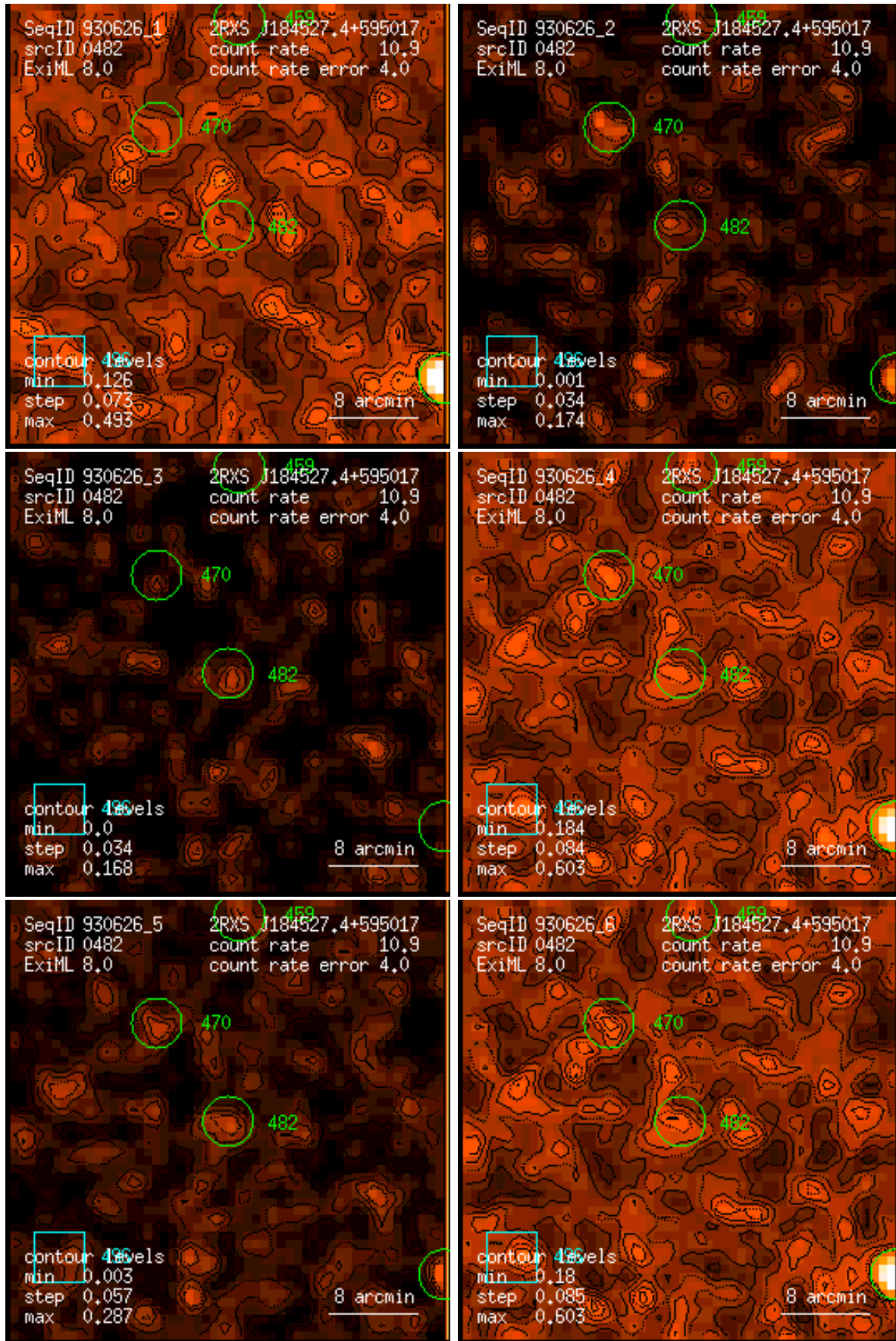
Figure 482: RASS 930626: detection 0482: band rate images, Gaussian filter: (1) PSPC channels 11 – 41, (2) 52 – 90, (3) 91 – 201, (4) 11 – 235, (5) 52 – 201, (6) 11 – 201. Broad band rates in counts/ks. Band rate contour levels in counts/ks/arcmin 2 .
