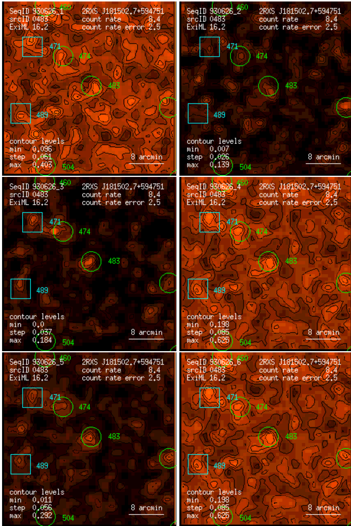
Figure 483: RASS 930626: detection 0483: band rate images, Gaussian filter: (1) PSPC channels 11 – 41, (2) 52 – 90, (3) 91 – 201, (4) 11 – 235, (5) 52 – 201, (6) 11 – 201. Broad band rates in counts/ks. Band rate contour levels in counts/ks/arcmin 2 .
