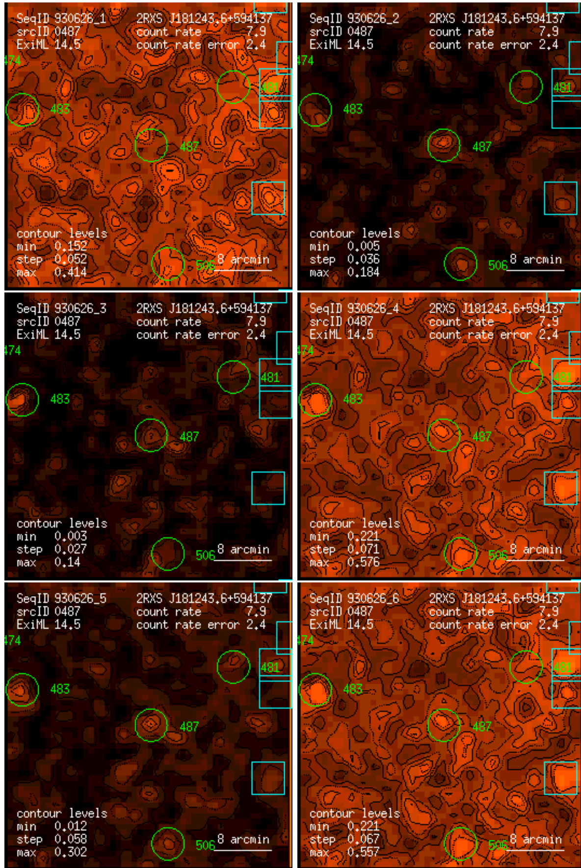
Figure 487: RASS 930626: detection 0487: band rate images, Gaussian filter: (1) PSPC channels 11 – 41, (2) 52 – 90, (3) 91 – 201, (4) 11 – 235, (5) 52 – 201, (6) 11 – 201. Broad band rates in counts/ks. Band rate contour levels in counts/ks/arcmin 2 .
