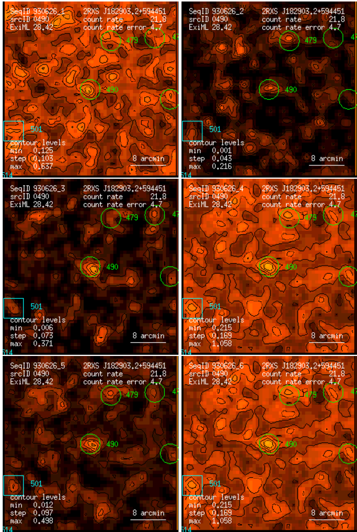
Figure 490: RASS 930626: detection 0490: band rate images, Gaussian filter: (1) PSPC channels 11 – 41, (2) 52 – 90, (3) 91 – 201, (4) 11 – 235, (5) 52 – 201, (6) 11 – 201. Broad band rates in counts/ks. Band rate contour levels in counts/ks/arcmin 2 .
