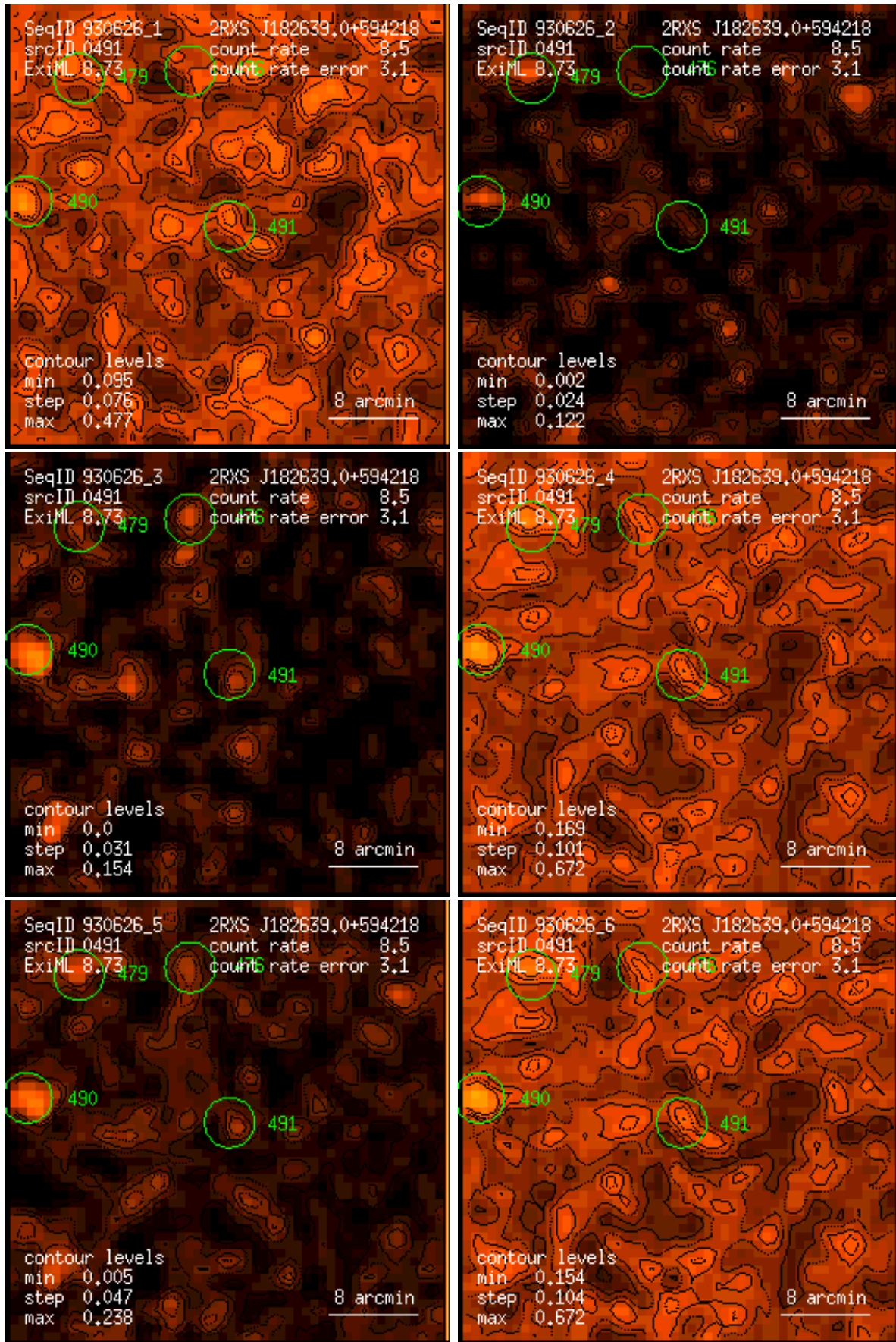
Figure 491: RASS 930626: detection 0491: band rate images, Gaussian filter: (1) PSPC channels 11 – 41, (2) 52 – 90, (3) 91 – 201, (4) 11 – 235, (5) 52 – 201, (6) 11 – 201. Broad band rates in counts/ks. Band rate contour levels in counts/ks/arcmin 2 .
