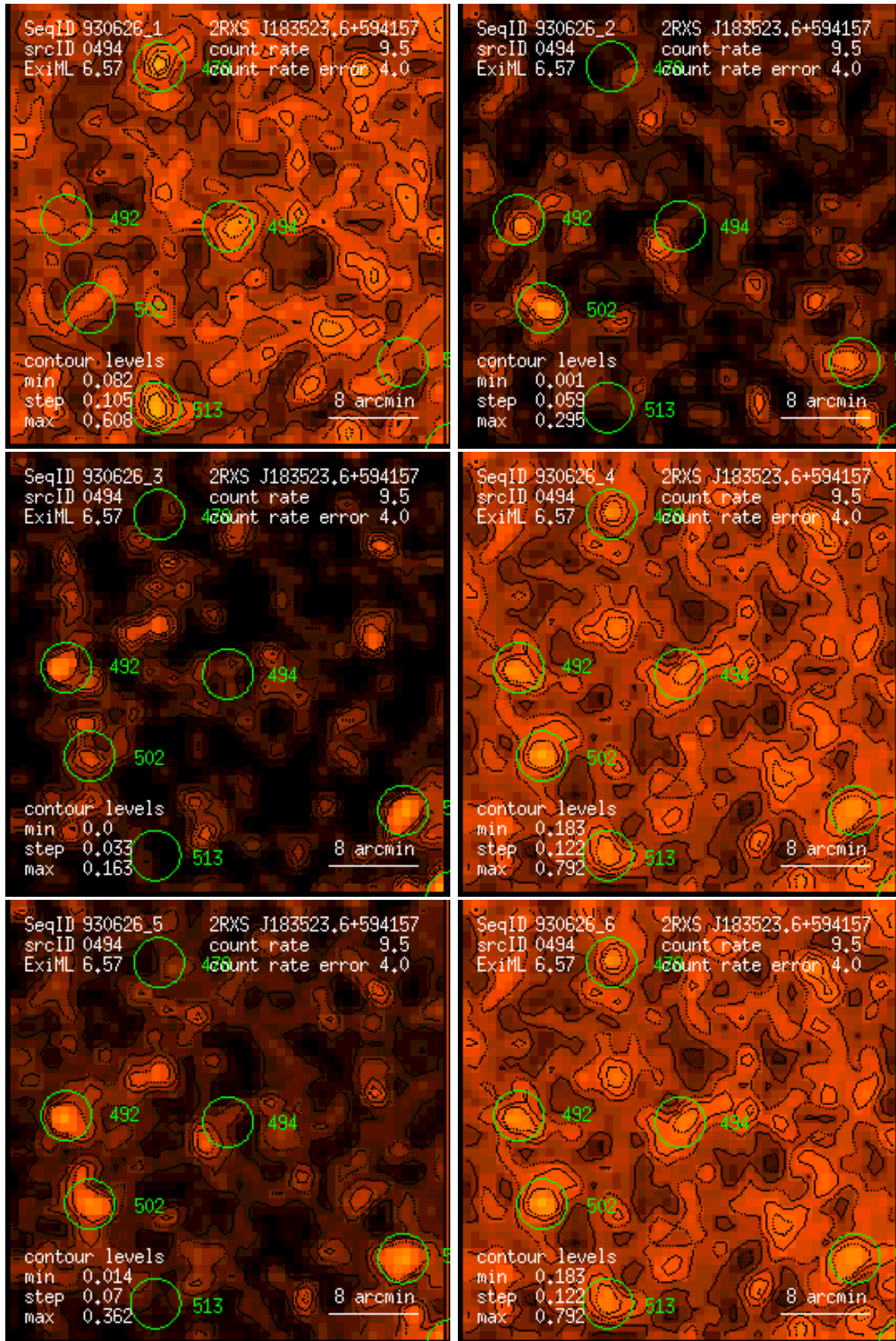
Figure 494: RASS 930626: detection 0494: band rate images, Gaussian filter: (1) PSPC channels 11 – 41, (2) 52 – 90, (3) 91 – 201, (4) 11 – 235, (5) 52 – 201, (6) 11 – 201. Broad band rates in counts/ks. Band rate contour levels in counts/ks/arcmin 2 .
