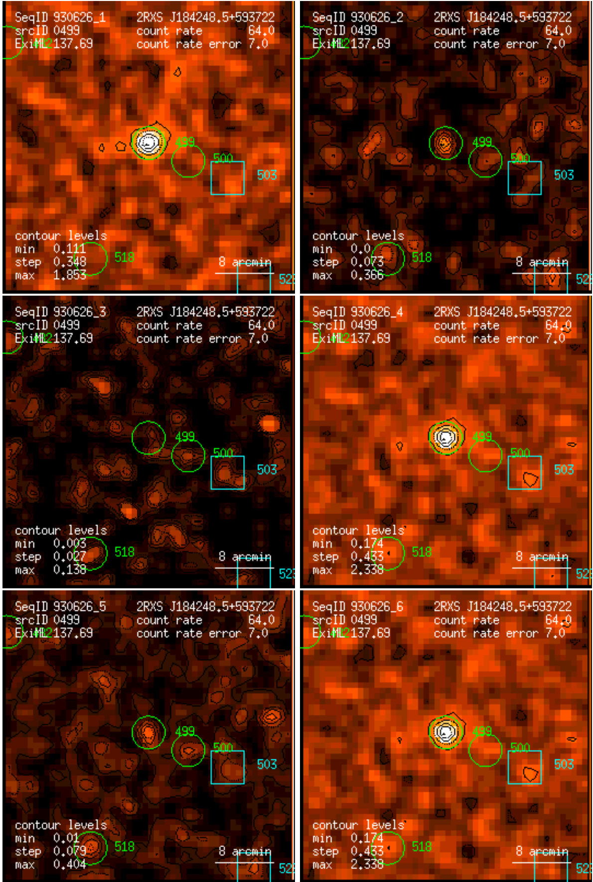
Figure 499: RASS 930626: detection 0499: band rate images, Gaussian filter: (1) PSPC channels 11 – 41, (2) 52 – 90, (3) 91 – 201, (4) 11 – 235, (5) 52 – 201, (6) 11 – 201. Broad band rates in counts/ks. Band rate contour levels in counts/ks/arcmin 2 .
