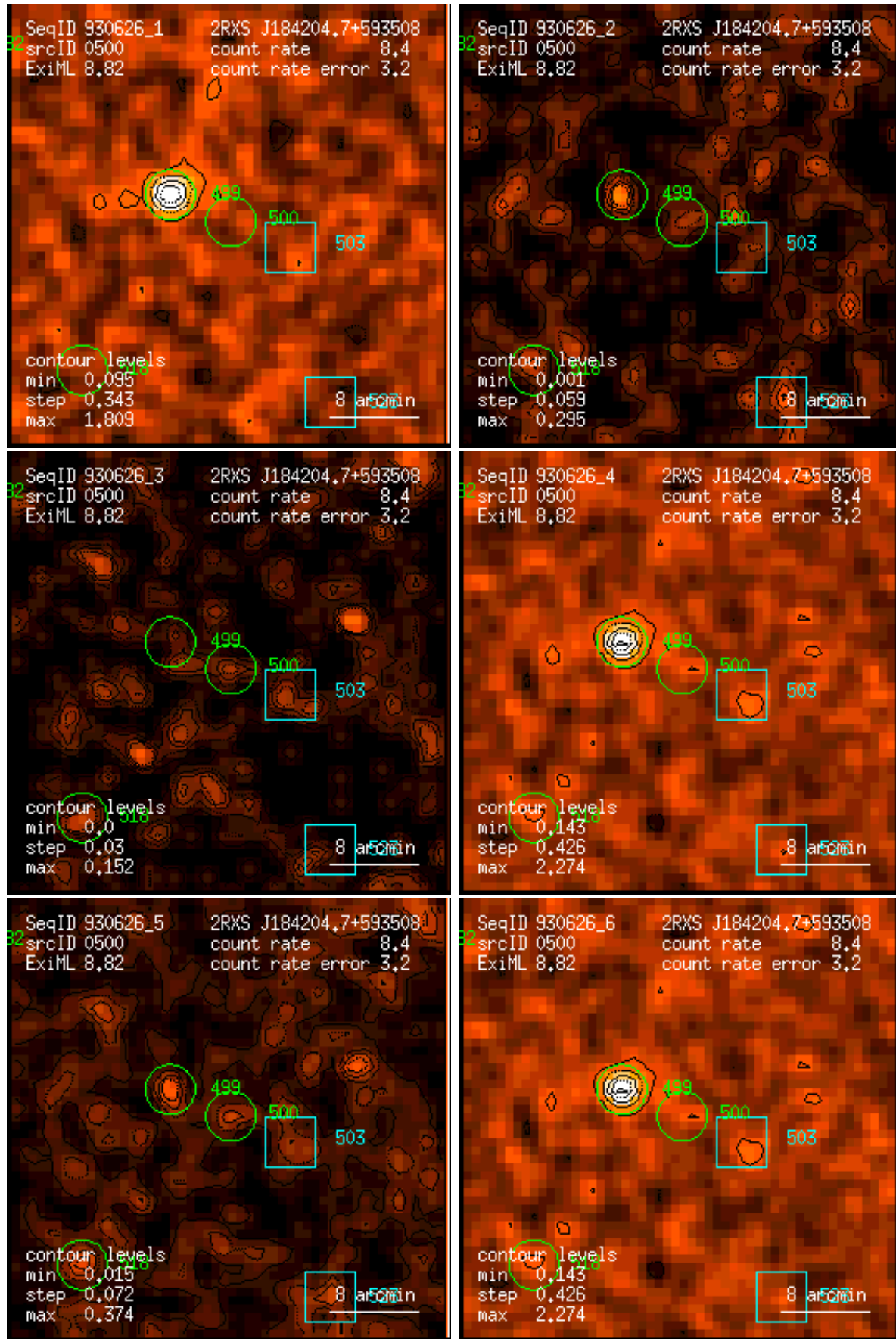
Figure 500: RASS 930626: detection 0500: band rate images, Gaussian filter: (1) PSPC channels 11 – 41, (2) 52 – 90, (3) 91 – 201, (4) 11 – 235, (5) 52 – 201, (6) 11 – 201. Broad band rates in counts/ks. Band rate contour levels in counts/ks/arcmin 2 .
