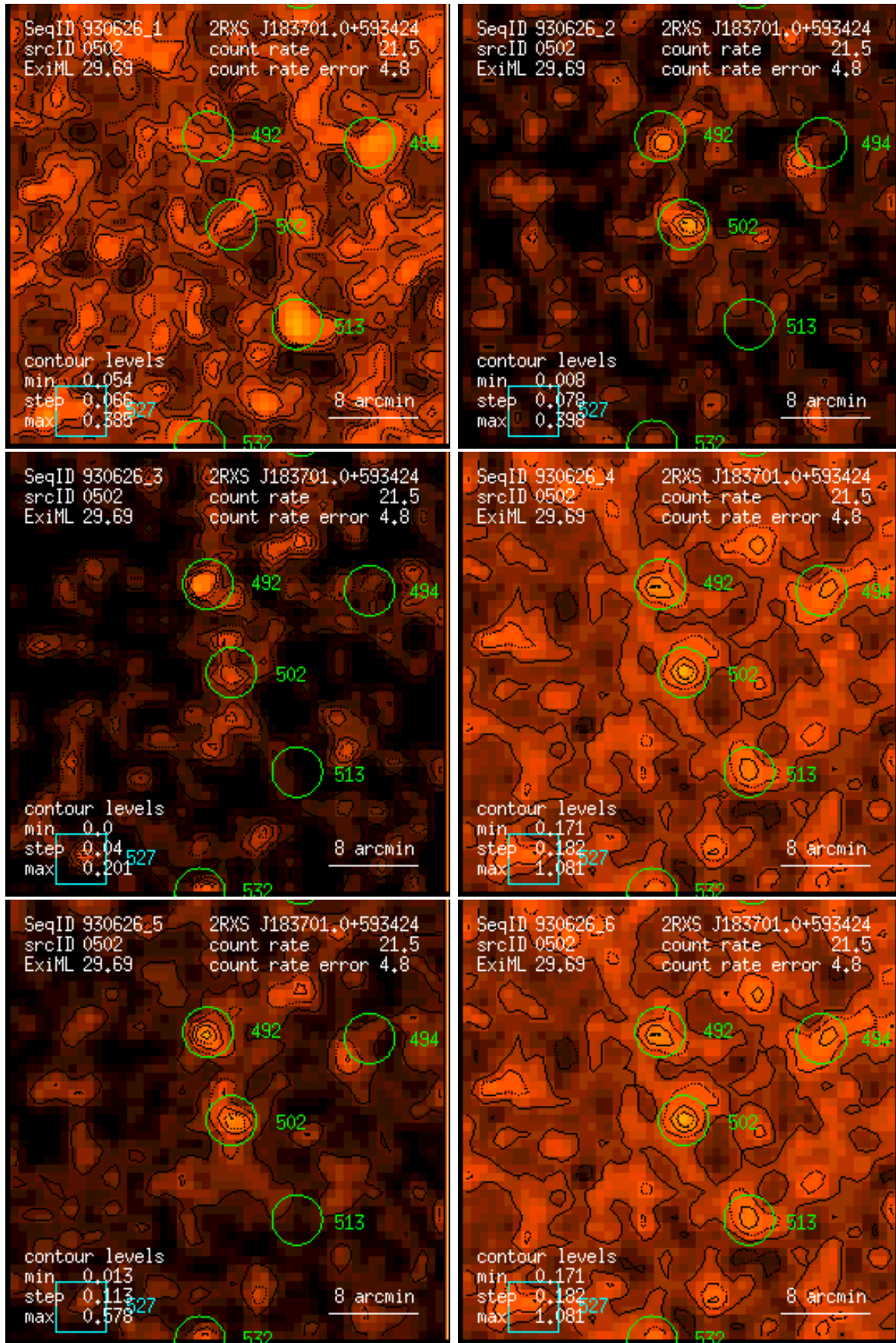
Figure 502: RASS 930626: detection 0502: band rate images, Gaussian filter: (1) PSPC channels 11 – 41, (2) 52 – 90, (3) 91 – 201, (4) 11 – 235, (5) 52 – 201, (6) 11 – 201. Broad band rates in counts/ks. Band rate contour levels in counts/ks/arcmin 2 .
