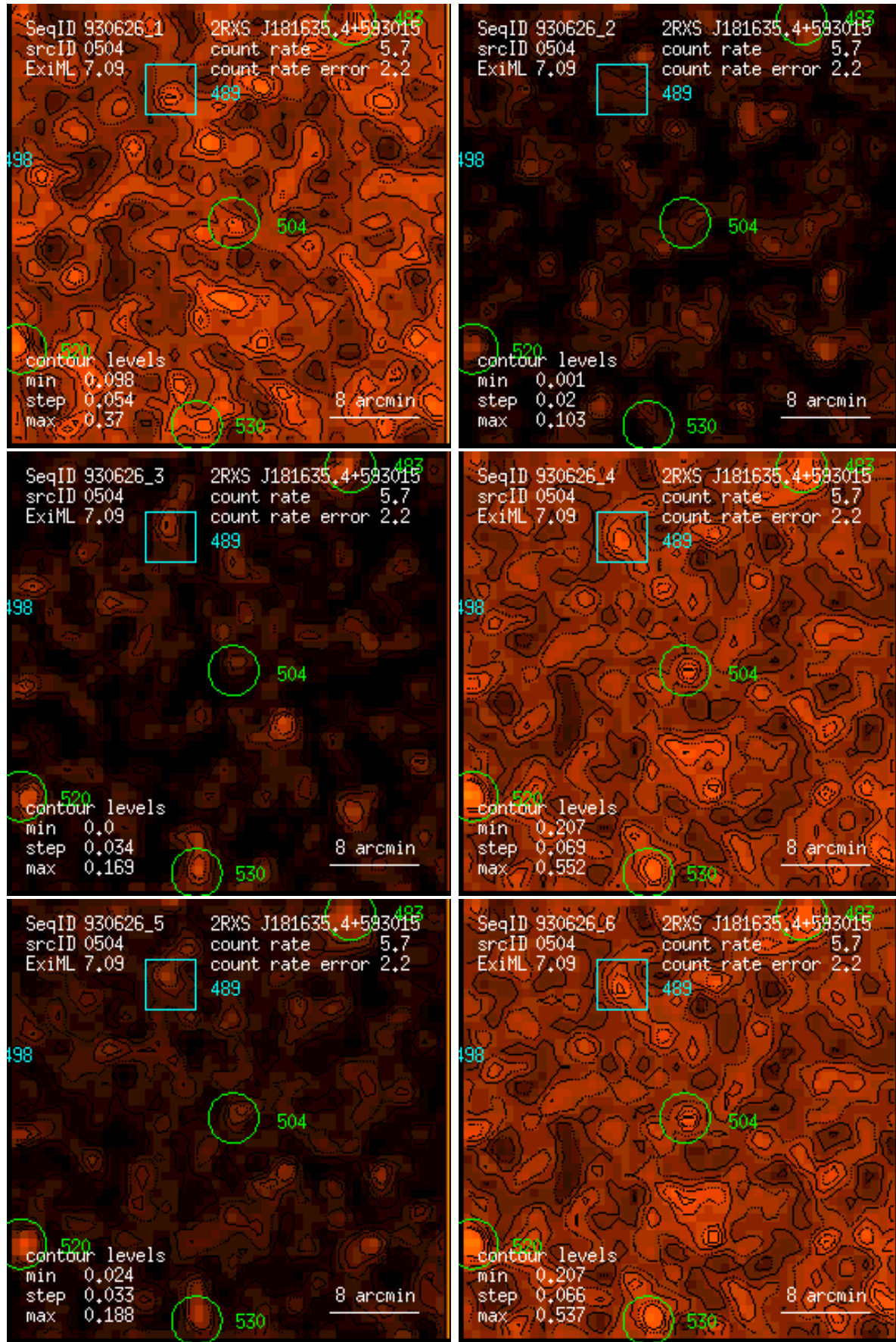
Figure 504: RASS 930626: detection 0504: band rate images, Gaussian filter: (1) PSPC channels 11 – 41, (2) 52 – 90, (3) 91 – 201, (4) 11 – 235, (5) 52 – 201, (6) 11 – 201. Broad band rates in counts/ks. Band rate contour levels in counts/ks/arcmin 2 .
