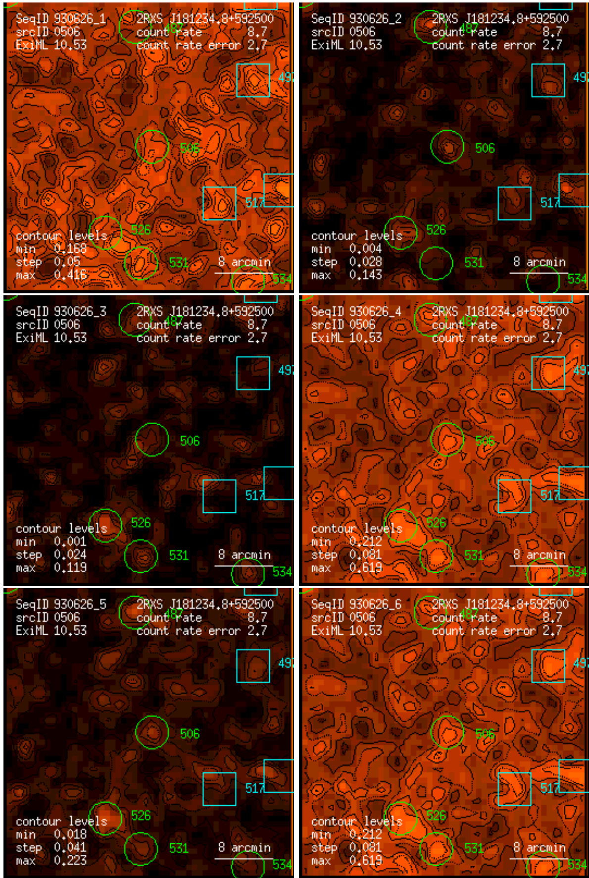
Figure 506: RASS 930626: detection 0506: band rate images, Gaussian filter: (1) PSPC channels 11 – 41, (2) 52 – 90, (3) 91 – 201, (4) 11 – 235, (5) 52 – 201, (6) 11 – 201. Broad band rates in counts/ks. Band rate contour levels in counts/ks/arcmin 2 .
