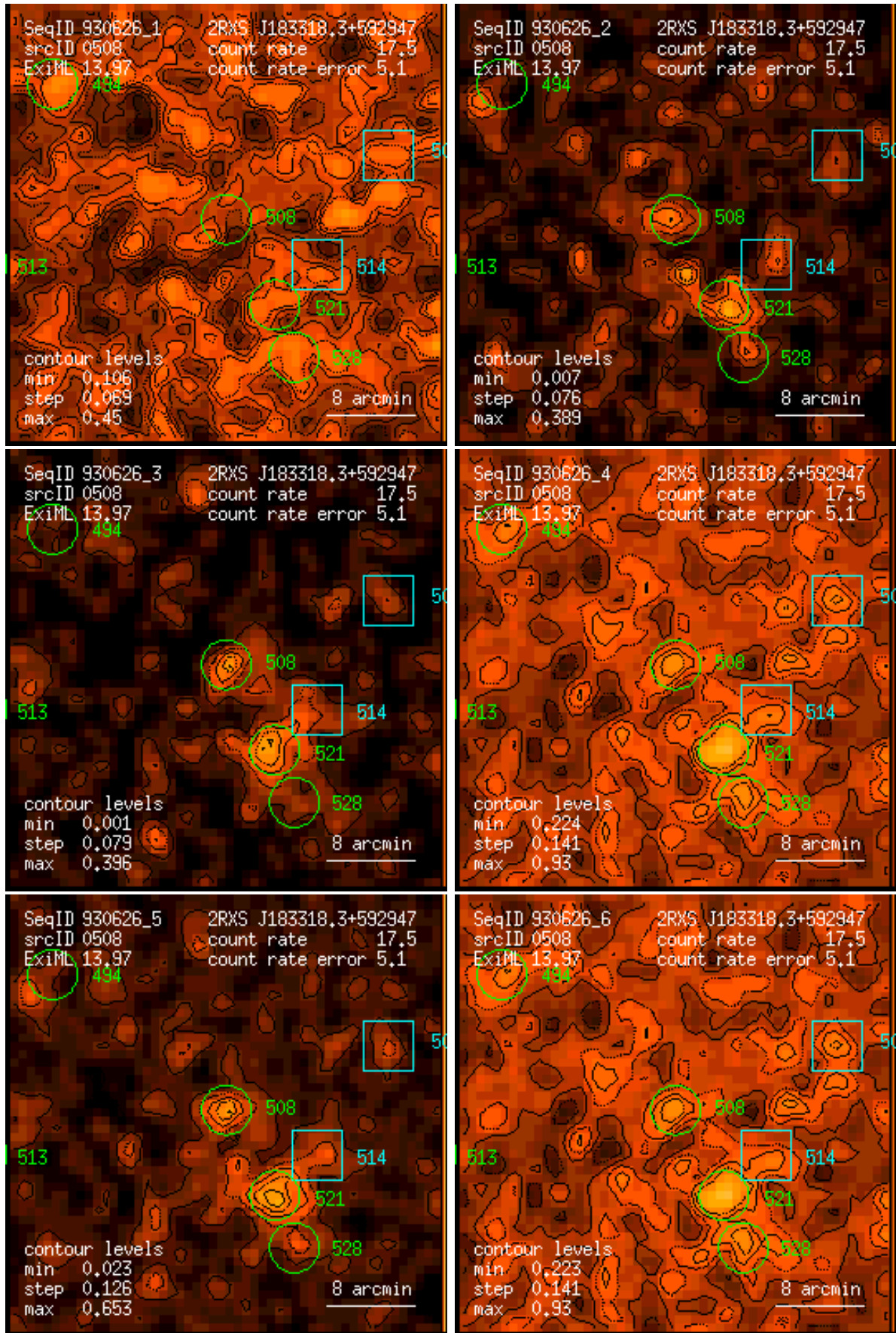
Figure 508: RASS 930626: detection 0508: band rate images, Gaussian filter: (1) PSPC channels 11 – 41, (2) 52 – 90, (3) 91 – 201, (4) 11 – 235, (5) 52 – 201, (6) 11 – 201. Broad band rates in counts/ks. Band rate contour levels in counts/ks/arcmin 2 .
