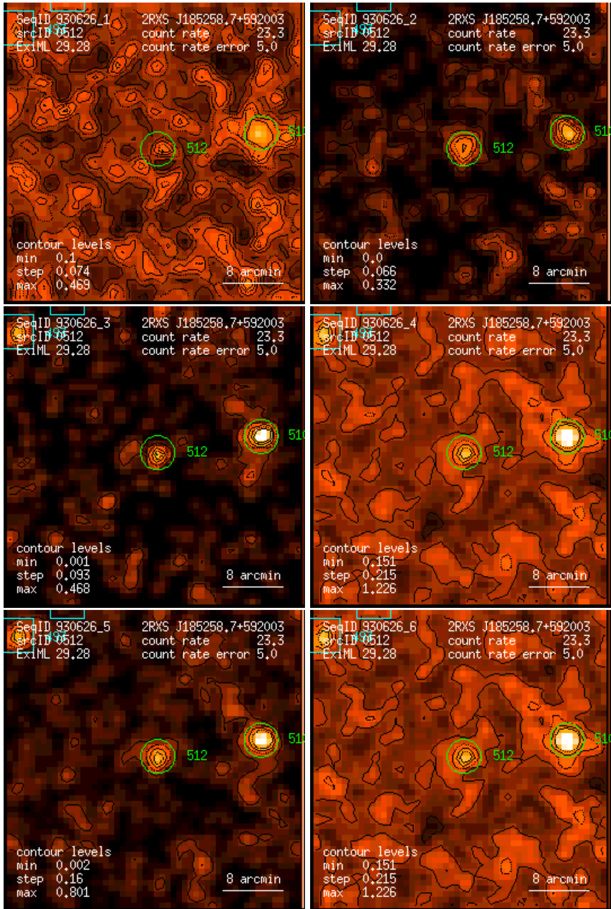
Figure 512: RASS 930626: detection 0512: band rate images, Gaussian filter: (1) PSPC channels 11 – 41, (2) 52 – 90, (3) 91 – 201, (4) 11 – 235, (5) 52 – 201, (6) 11 – 201. Broad band rates in counts/ks. Band rate contour levels in counts/ks/arcmin 2 .
