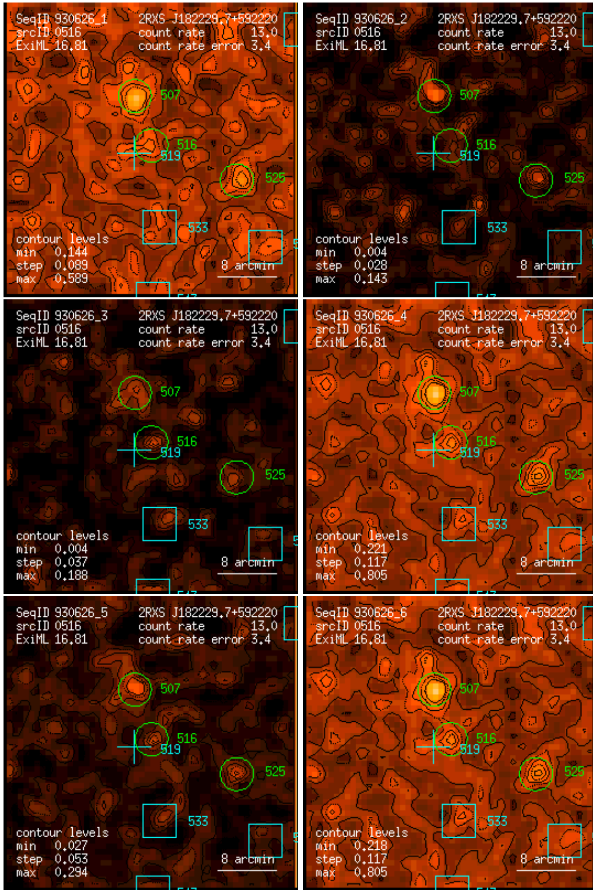
Figure 516: RASS 930626: detection 0516: band rate images, Gaussian filter: (1) PSPC channels 11 – 41, (2) 52 – 90, (3) 91 – 201, (4) 11 – 235, (5) 52 – 201, (6) 11 – 201. Broad band rates in counts/ks. Band rate contour levels in counts/ks/arcmin 2 .
