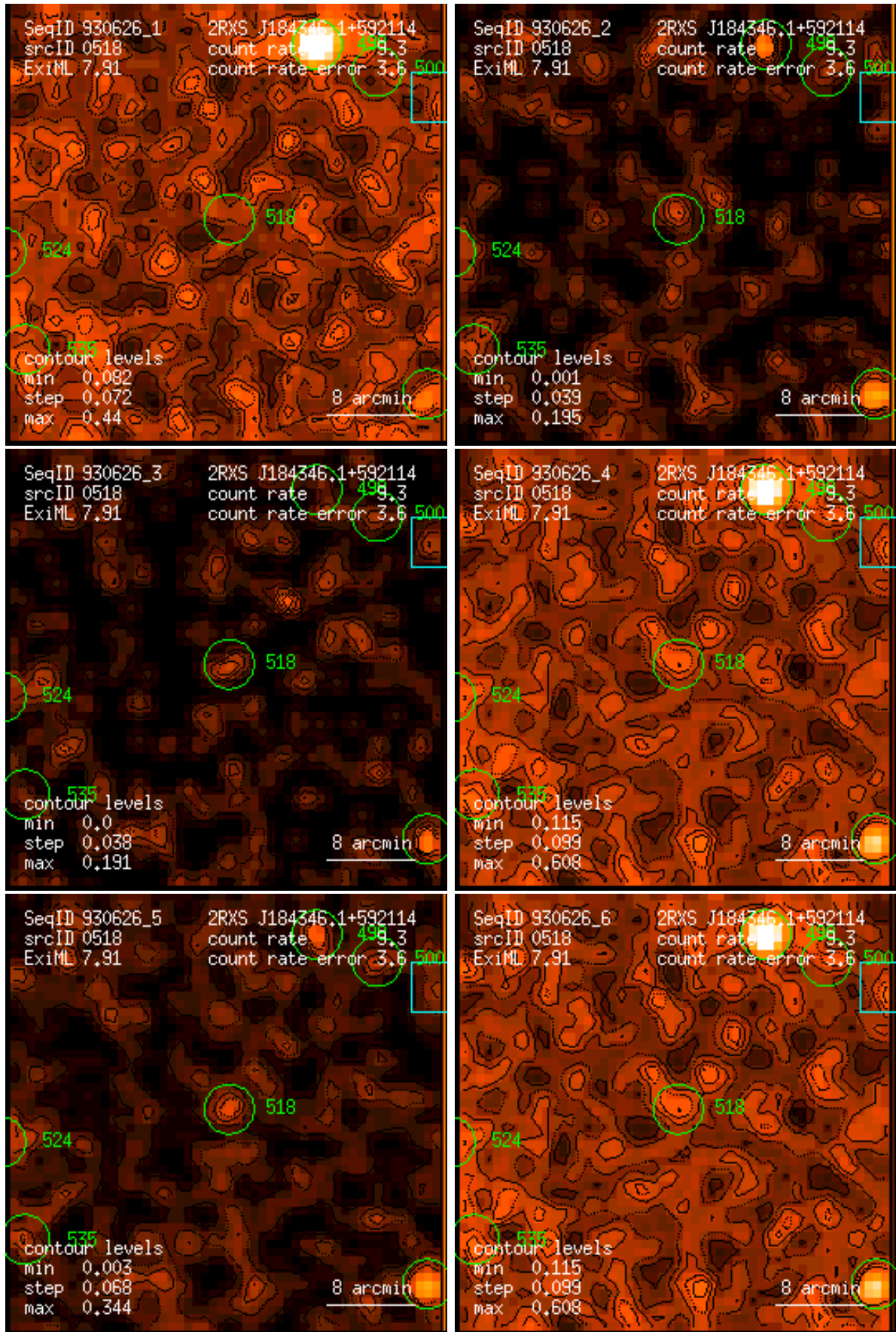
Figure 518: RASS 930626: detection 0518: band rate images, Gaussian filter: (1) PSPC channels 11 – 41, (2) 52 – 90, (3) 91 – 201, (4) 11 – 235, (5) 52 – 201, (6) 11 – 201. Broad band rates in counts/ks. Band rate contour levels in counts/ks/arcmin 2 .
