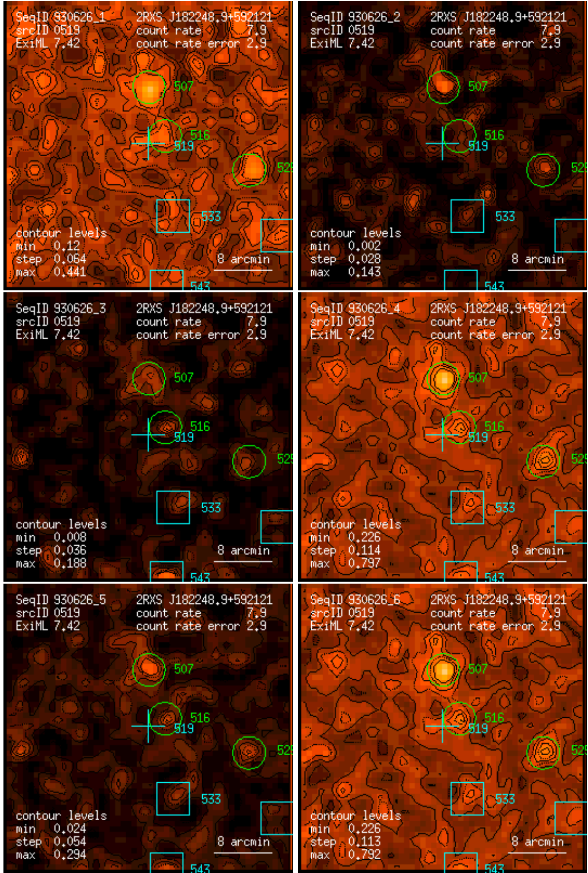
Figure 519: RASS 930626: detection 0519: band rate images, Gaussian filter: (1) PSPC channels 11 – 41, (2) 52 – 90, (3) 91 – 201, (4) 11 – 235, (5) 52 – 201, (6) 11 – 201. Broad band rates in counts/ks. Band rate contour levels in counts/ks/arcmin 2 .
