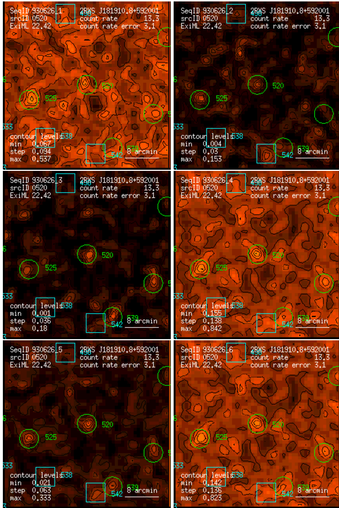
Figure 520: RASS 930626: detection 0520: band rate images, Gaussian filter: (1) PSPC channels 11 – 41, (2) 52 – 90, (3) 91 – 201, (4) 11 – 235, (5) 52 – 201, (6) 11 – 201. Broad band rates in counts/ks. Band rate contour levels in counts/ks/arcmin 2 .
