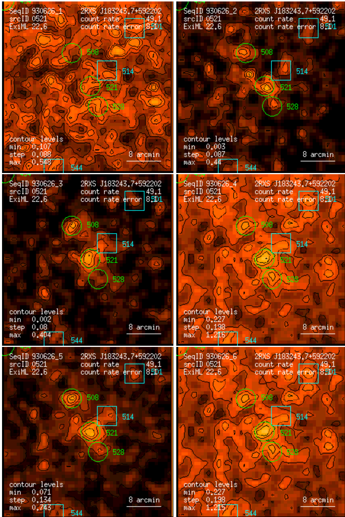
Figure 521: RASS 930626: detection 0521: band rate images, Gaussian filter: (1) PSPC channels 11 – 41, (2) 52 – 90, (3) 91 – 201, (4) 11 – 235, (5) 52 – 201, (6) 11 – 201. Broad band rates in counts/ks. Band rate contour levels in counts/ks/arcmin 2 .
