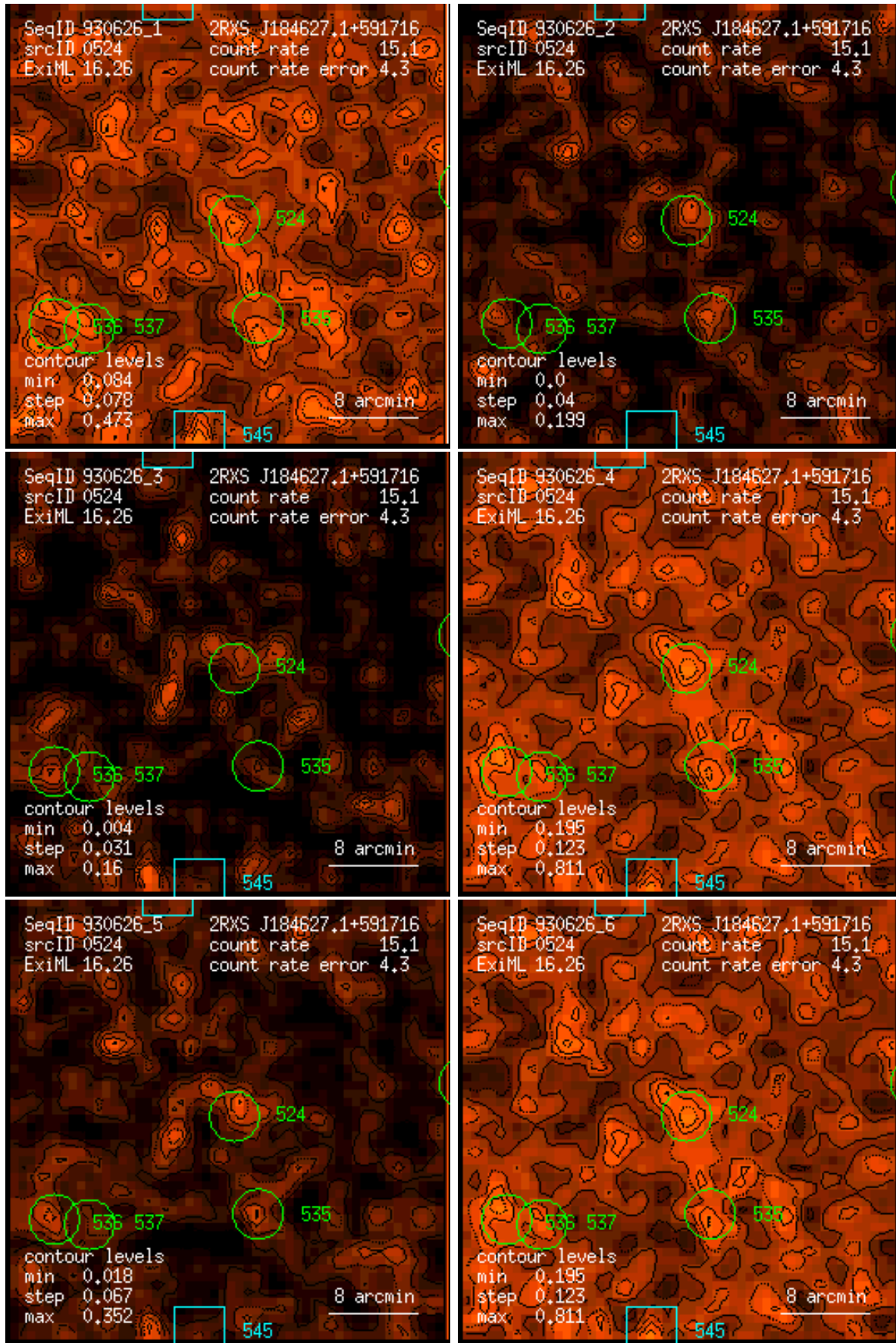
Figure 524: RASS 930626: detection 0524: band rate images, Gaussian filter: (1) PSPC channels 11 – 41, (2) 52 – 90, (3) 91 – 201, (4) 11 – 235, (5) 52 – 201, (6) 11 – 201. Broad band rates in counts/ks. Band rate contour levels in counts/ks/arcmin 2 .
