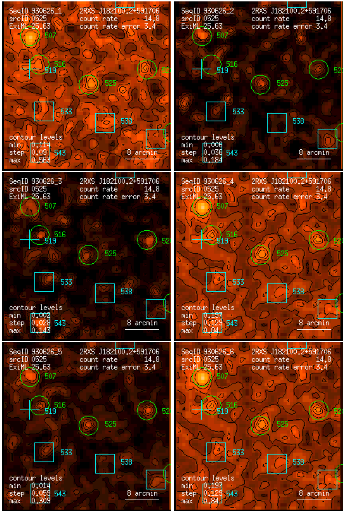
Figure 525: RASS 930626: detection 0525: band rate images, Gaussian filter: (1) PSPC channels 11 – 41, (2) 52 – 90, (3) 91 – 201, (4) 11 – 235, (5) 52 – 201, (6) 11 – 201. Broad band rates in counts/ks. Band rate contour levels in counts/ks/arcmin 2 .
