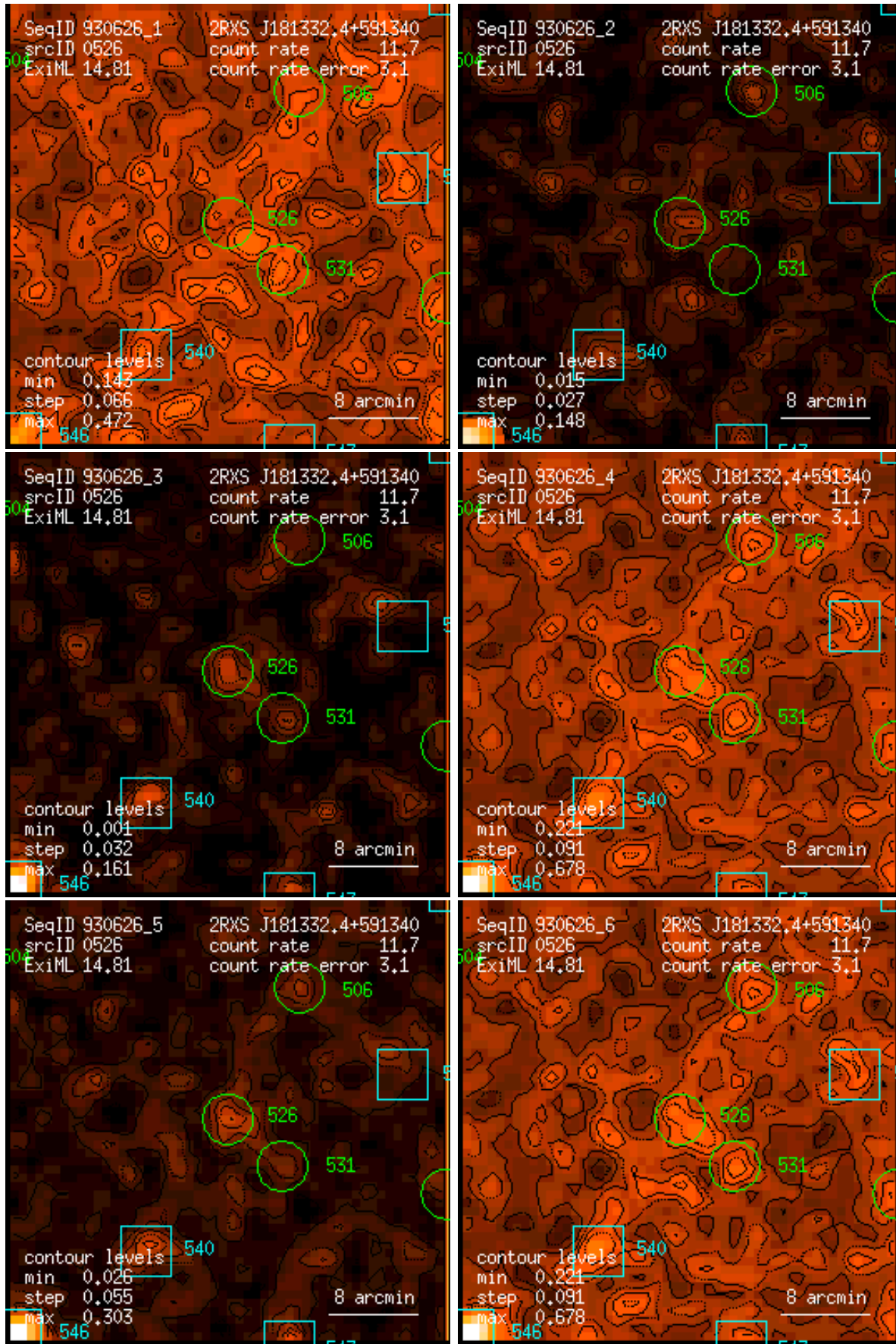
Figure 526: RASS 930626: detection 0526: band rate images, Gaussian filter: (1) PSPC channels 11 – 41, (2) 52 – 90, (3) 91 – 201, (4) 11 – 235, (5) 52 – 201, (6) 11 – 201. Broad band rates in counts/ks. Band rate contour levels in counts/ks/arcmin 2 .
