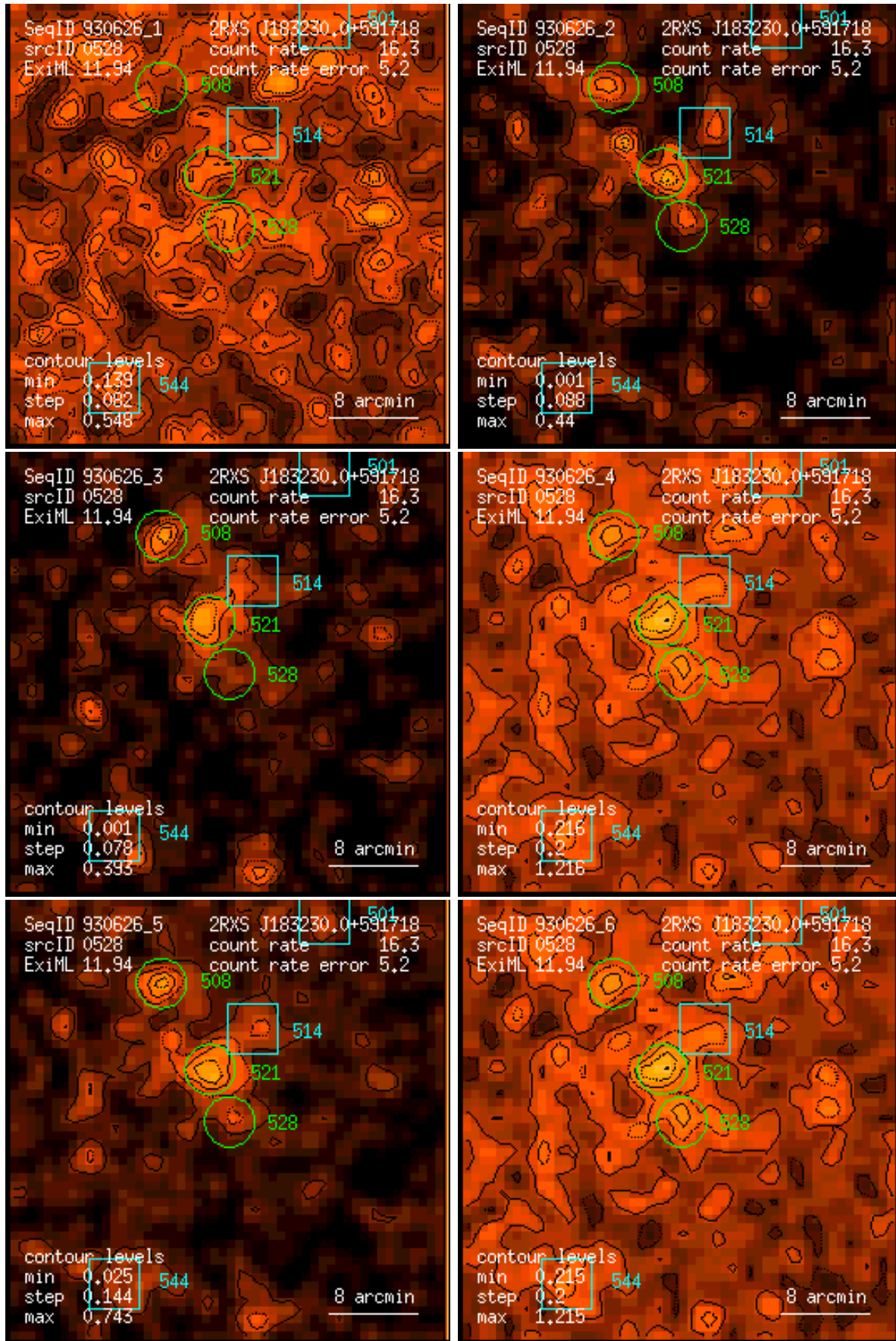
Figure 528: RASS 930626: detection 0528: band rate images, Gaussian filter: (1) PSPC channels 11 – 41, (2) 52 – 90, (3) 91 – 201, (4) 11 – 235, (5) 52 – 201, (6) 11 – 201. Broad band rates in counts/ks. Band rate contour levels in counts/ks/arcmin 2 .
