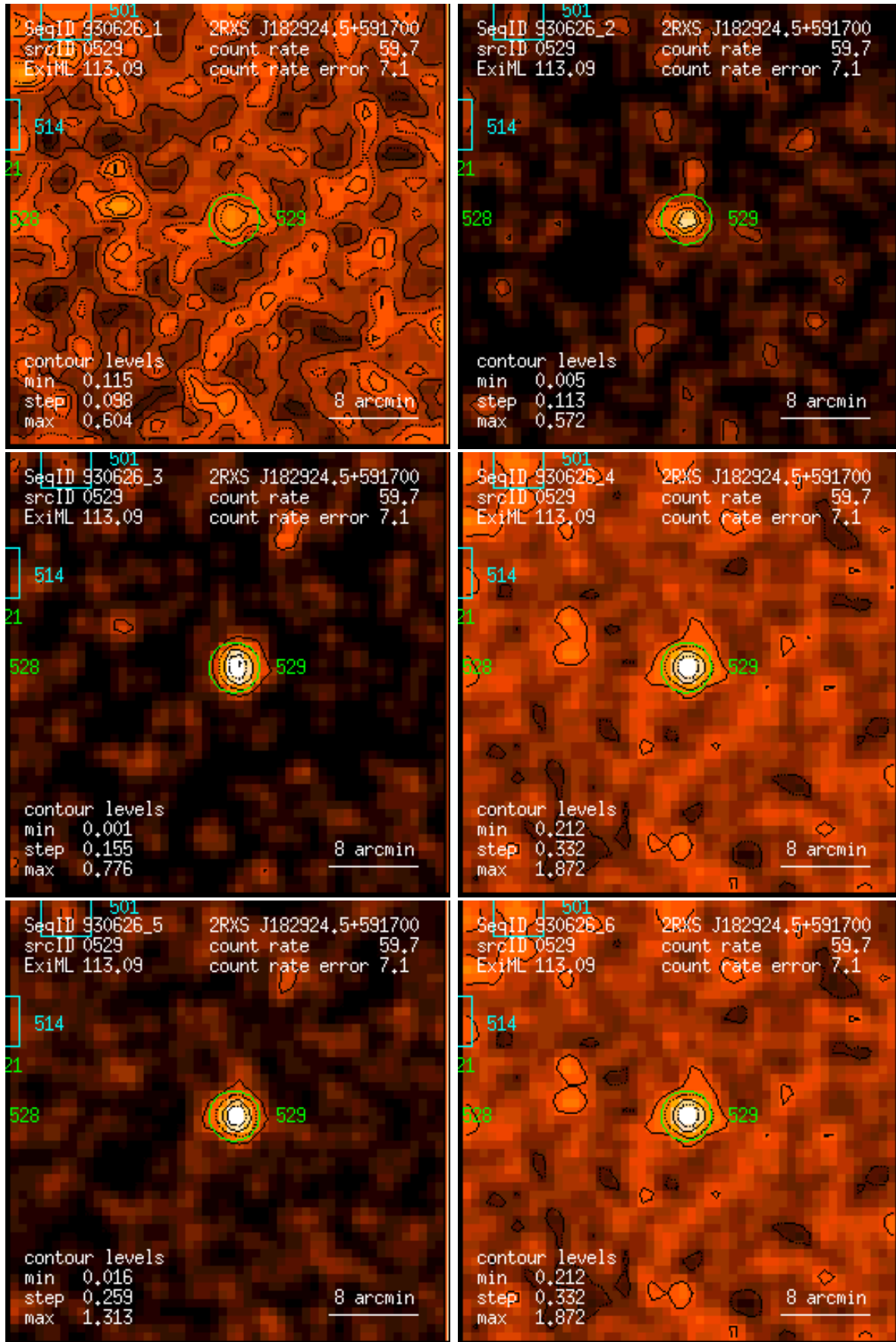
Figure 529: RASS 930626: detection 0529: band rate images, Gaussian filter: (1) PSPC channels 11 – 41, (2) 52 – 90, (3) 91 – 201, (4) 11 – 235, (5) 52 – 201, (6) 11 – 201. Broad band rates in counts/ks. Band rate contour levels in counts/ks/arcmin 2 .
