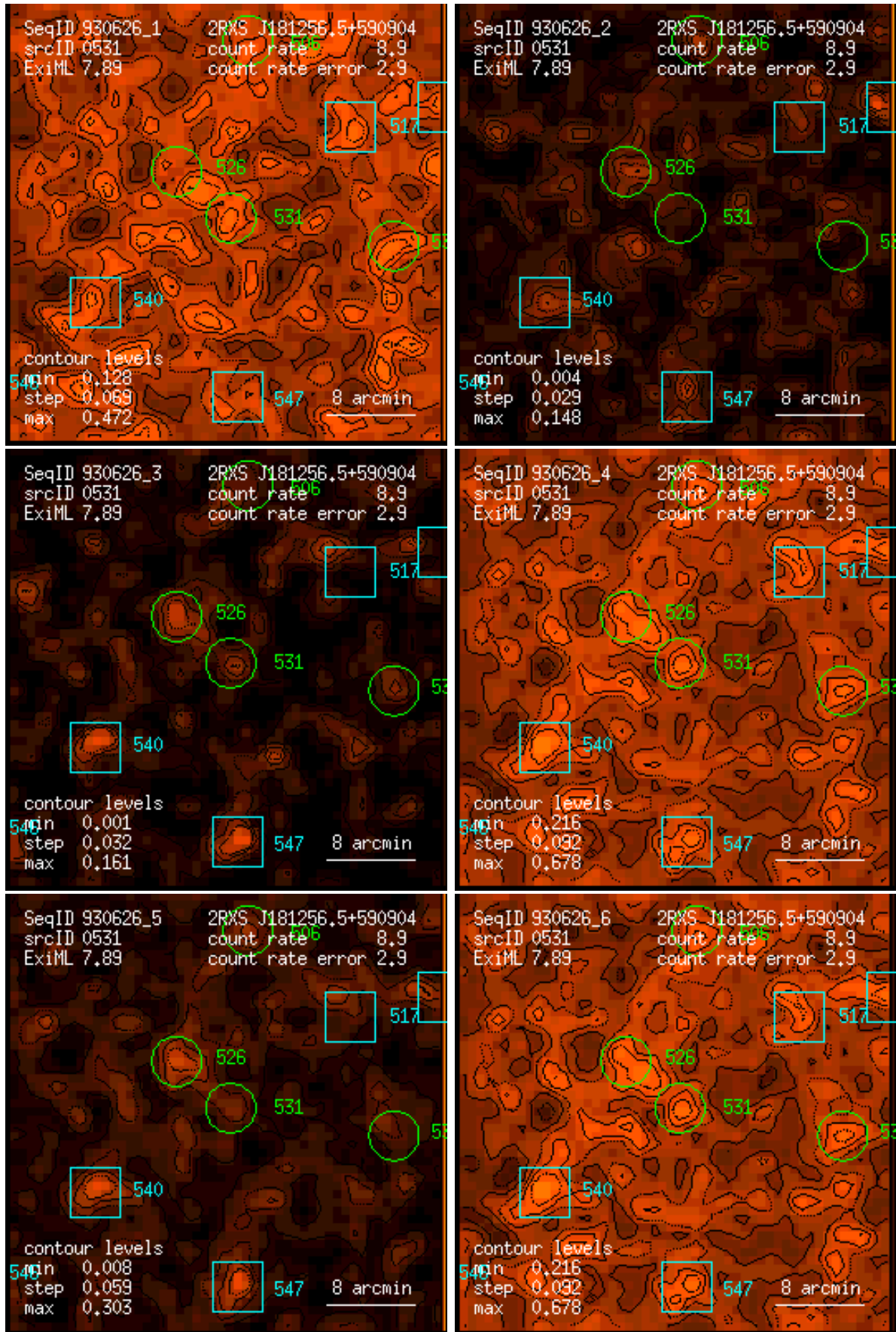
Figure 531: RASS 930626: detection 0531: band rate images, Gaussian filter: (1) PSPC channels 11 – 41, (2) 52 – 90, (3) 91 – 201, (4) 11 – 235, (5) 52 – 201, (6) 11 – 201. Broad band rates in counts/ks. Band rate contour levels in counts/ks/arcmin 2 .
