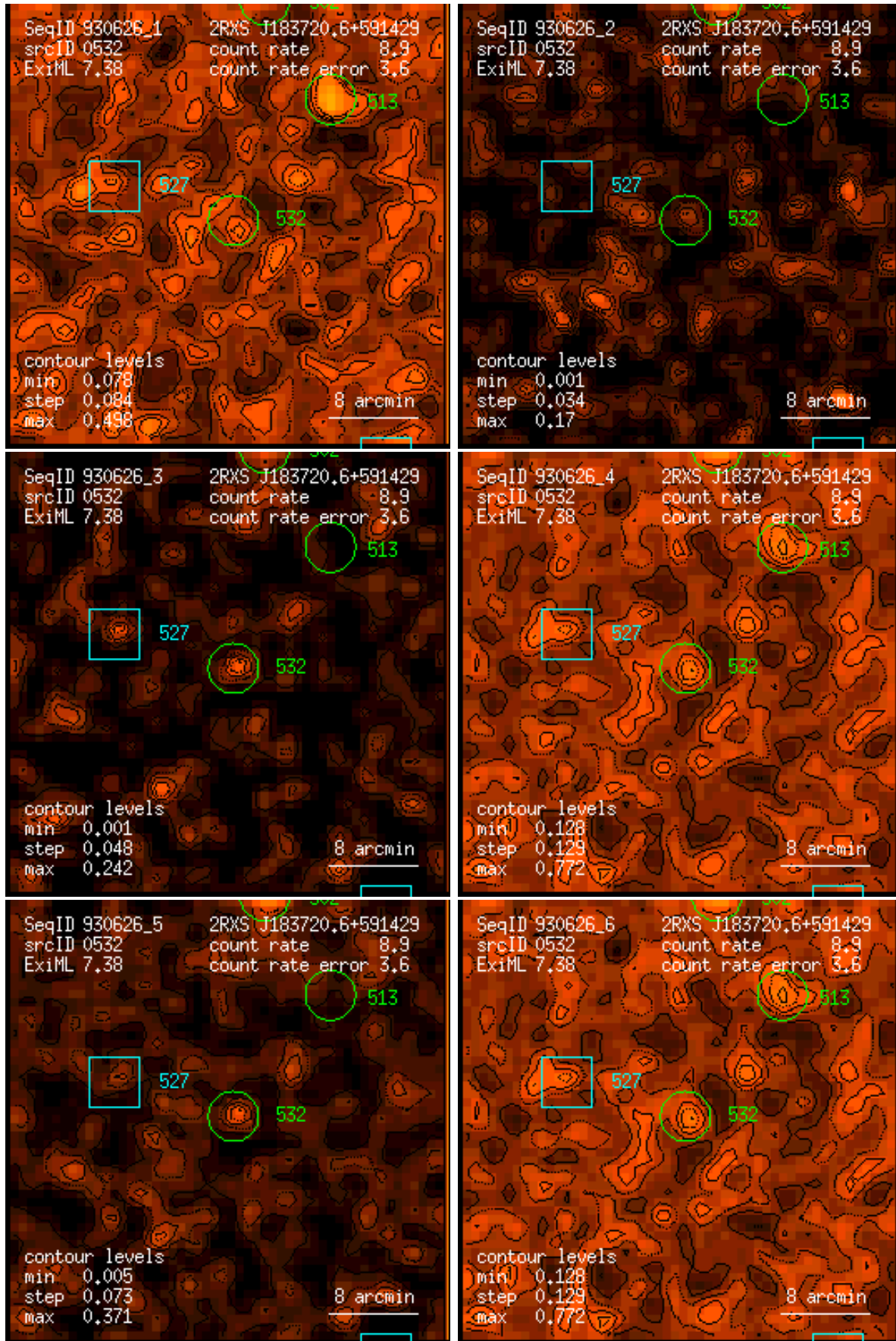
Figure 532: RASS 930626: detection 0532: band rate images, Gaussian filter: (1) PSPC channels 11 – 41, (2) 52 – 90, (3) 91 – 201, (4) 11 – 235, (5) 52 – 201, (6) 11 – 201. Broad band rates in counts/ks. Band rate contour levels in counts/ks/arcmin 2 .
