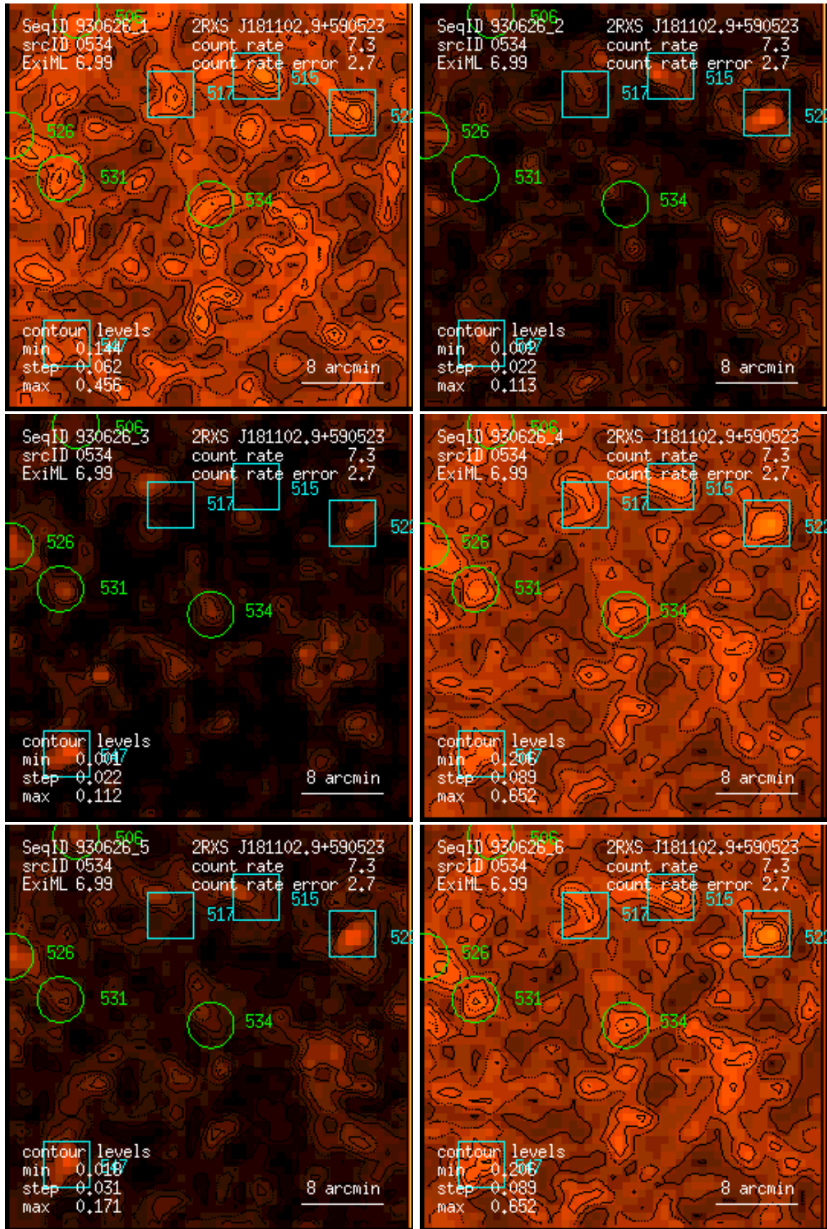
Figure 534: RASS 930626: detection 0534: band rate images, Gaussian filter: (1) PSPC channels 11 – 41, (2) 52 – 90, (3) 91 – 201, (4) 11 – 235, (5) 52 – 201, (6) 11 – 201. Broad band rates in counts/ks. Band rate contour levels in counts/ks/arcmin 2 .
