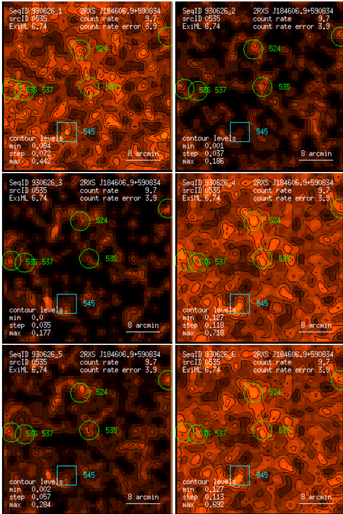
Figure 535: RASS 930626: detection 0535: band rate images, Gaussian filter: (1) PSPC channels 11 – 41, (2) 52 – 90, (3) 91 – 201, (4) 11 – 235, (5) 52 – 201, (6) 11 – 201. Broad band rates in counts/ks. Band rate contour levels in counts/ks/arcmin 2 .
