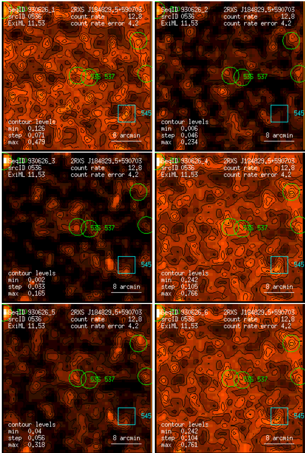
Figure 536: RASS 930626: detection 0536: band rate images, Gaussian filter: (1) PSPC channels 11 – 41, (2) 52 – 90, (3) 91 – 201, (4) 11 – 235, (5) 52 – 201, (6) 11 – 201. Broad band rates in counts/ks. Band rate contour levels in counts/ks/arcmin 2 .
