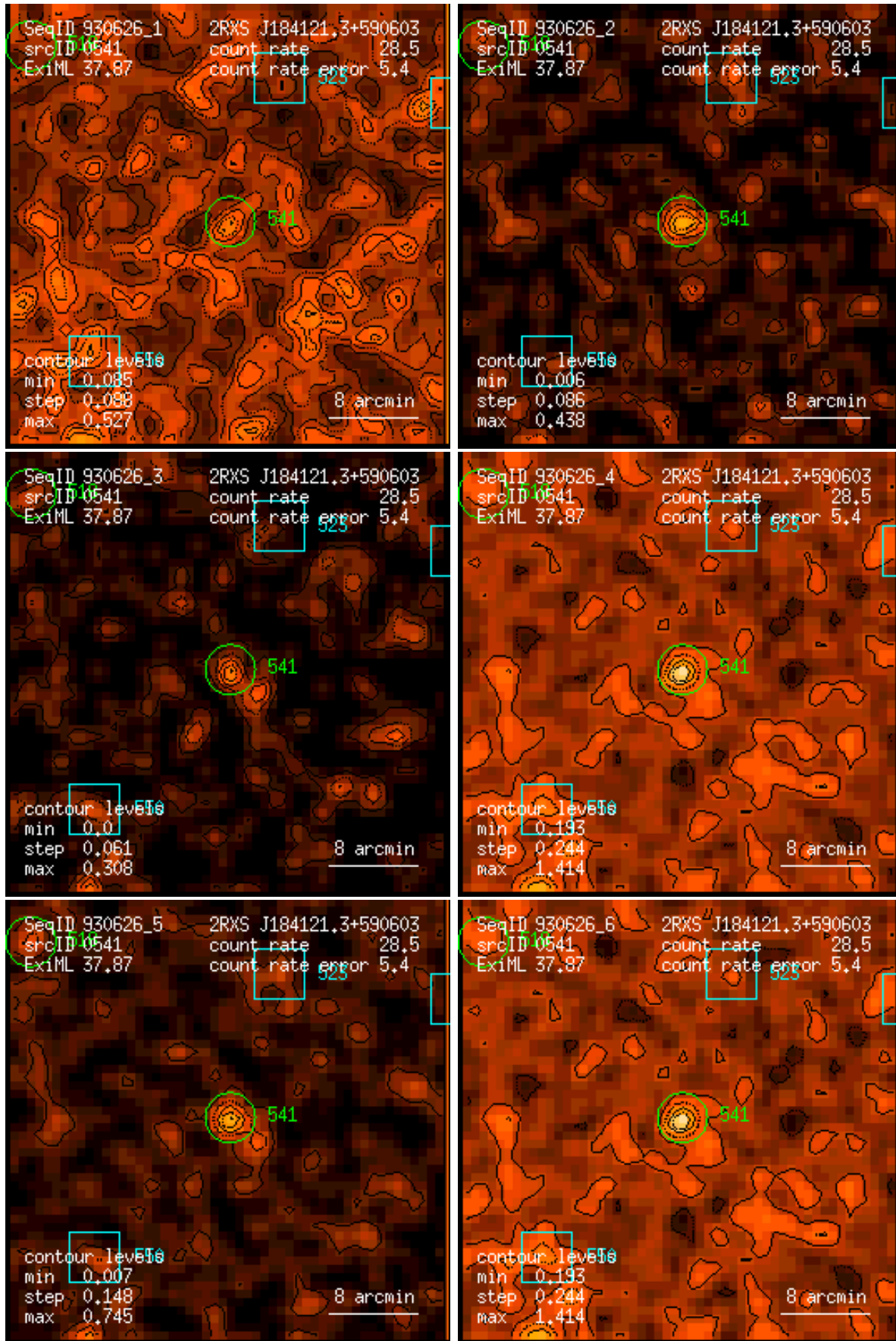
Figure 541: RASS 930626: detection 0541: band rate images, Gaussian filter: (1) PSPC channels 11 – 41, (2) 52 – 90, (3) 91 – 201, (4) 11 – 235, (5) 52 – 201, (6) 11 – 201. Broad band rates in counts/ks. Band rate contour levels in counts/ks/arcmin 2 .
