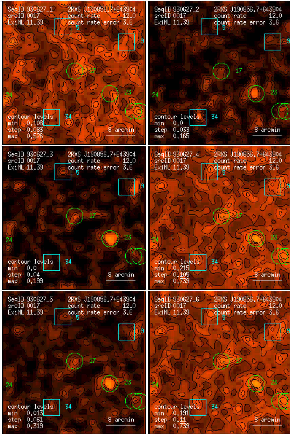
Figure 17: RASS 930627: detection 0017: band rate images, Gaussian filter: (1) PSPC channels 11 – 41, (2) 52 – 90, (3) 91 – 201, (4) 11 – 235, (5) 52 – 201, (6) 11 – 201. Broad band rates in counts/ks. Band rate contour levels in counts/ks/arcmin 2 .
