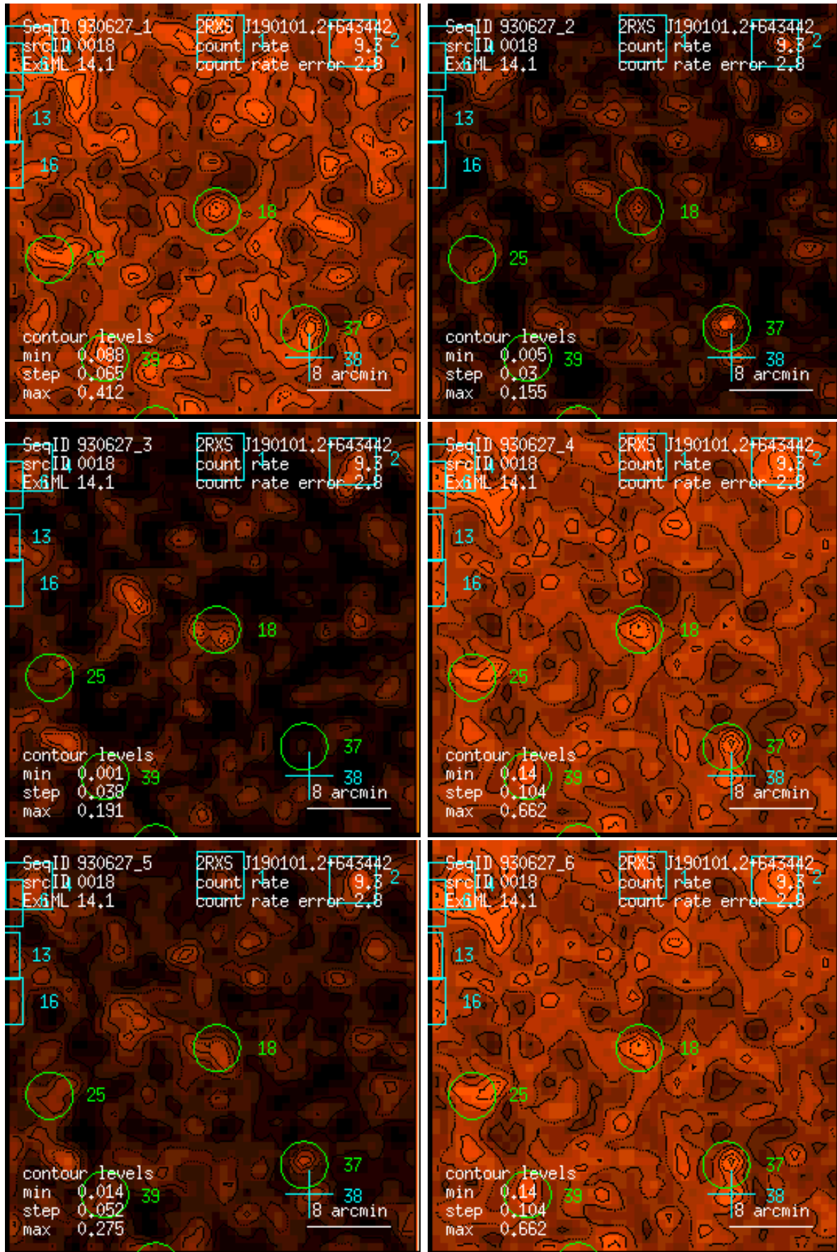
Figure 18: RASS 930627: detection 0018: band rate images, Gaussian filter: (1) PSPC channels 11 – 41, (2) 52 – 90, (3) 91 – 201, (4) 11 – 235, (5) 52 – 201, (6) 11 – 201. Broad band rates in counts/ks. Band rate contour levels in counts/ks/arcmin 2 .
