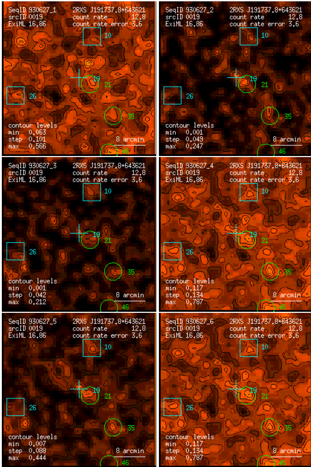
Figure 19: RASS 930627: detection 0019: band rate images, Gaussian filter: (1) PSPC channels 11 – 41, (2) 52 – 90, (3) 91 – 201, (4) 11 – 235, (5) 52 – 201, (6) 11 – 201. Broad band rates in counts/ks. Band rate contour levels in counts/ks/arcmin 2 .
