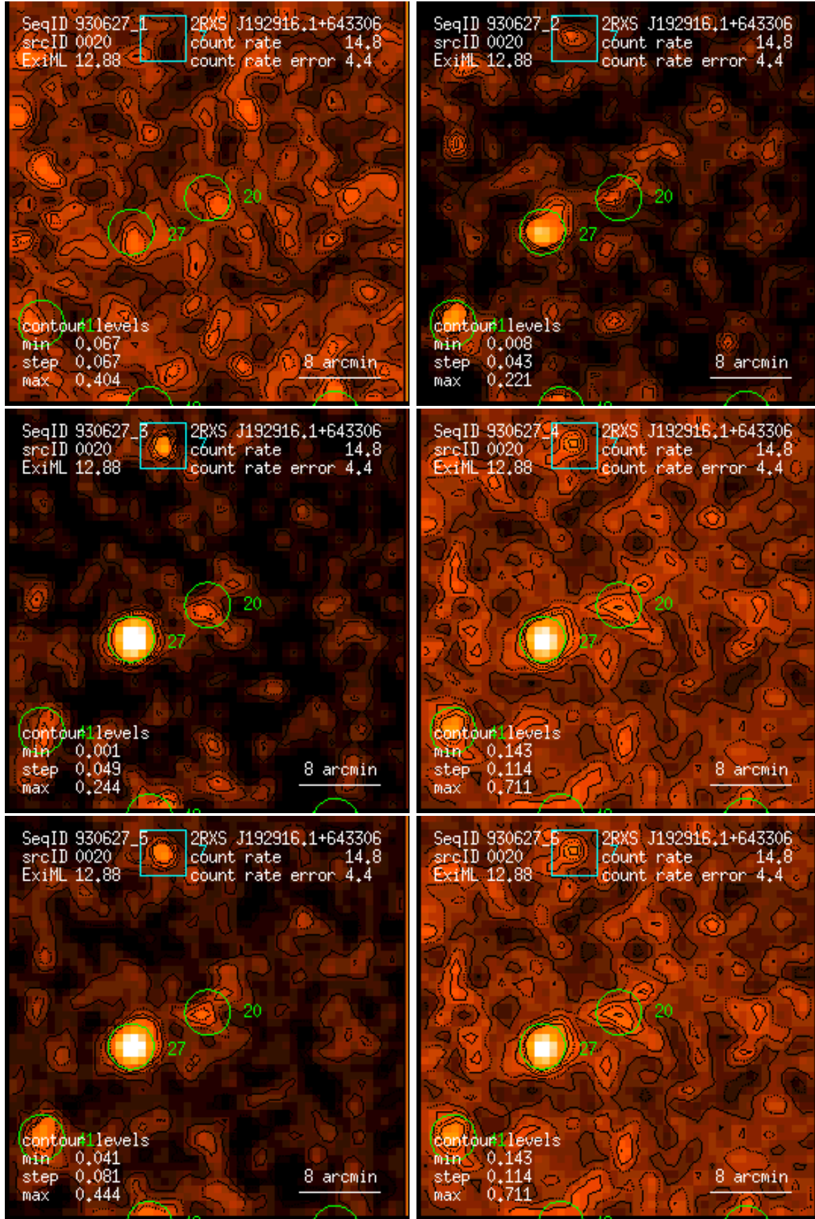
Figure 20: RASS 930627: detection 0020: band rate images, Gaussian filter: (1) PSPC channels 11 – 41, (2) 52 – 90, (3) 91 – 201, (4) 11 – 235, (5) 52 – 201, (6) 11 – 201. Broad band rates in counts/ks. Band rate contour levels in counts/ks/arcmin 2 .
