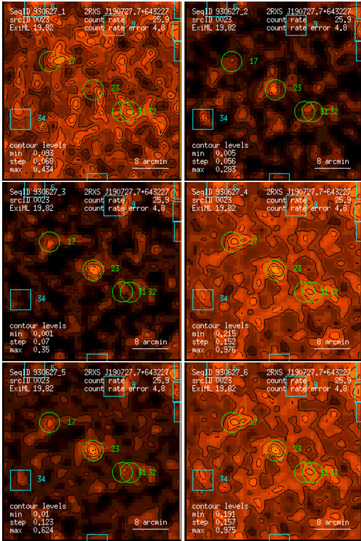
Figure 23: RASS 930627: detection 0023: band rate images, Gaussian filter: (1) PSPC channels 11 – 41, (2) 52 – 90, (3) 91 – 201, (4) 11 – 235, (5) 52 – 201, (6) 11 – 201. Broad band rates in counts/ks. Band rate contour levels in counts/ks/arcmin 2 .
