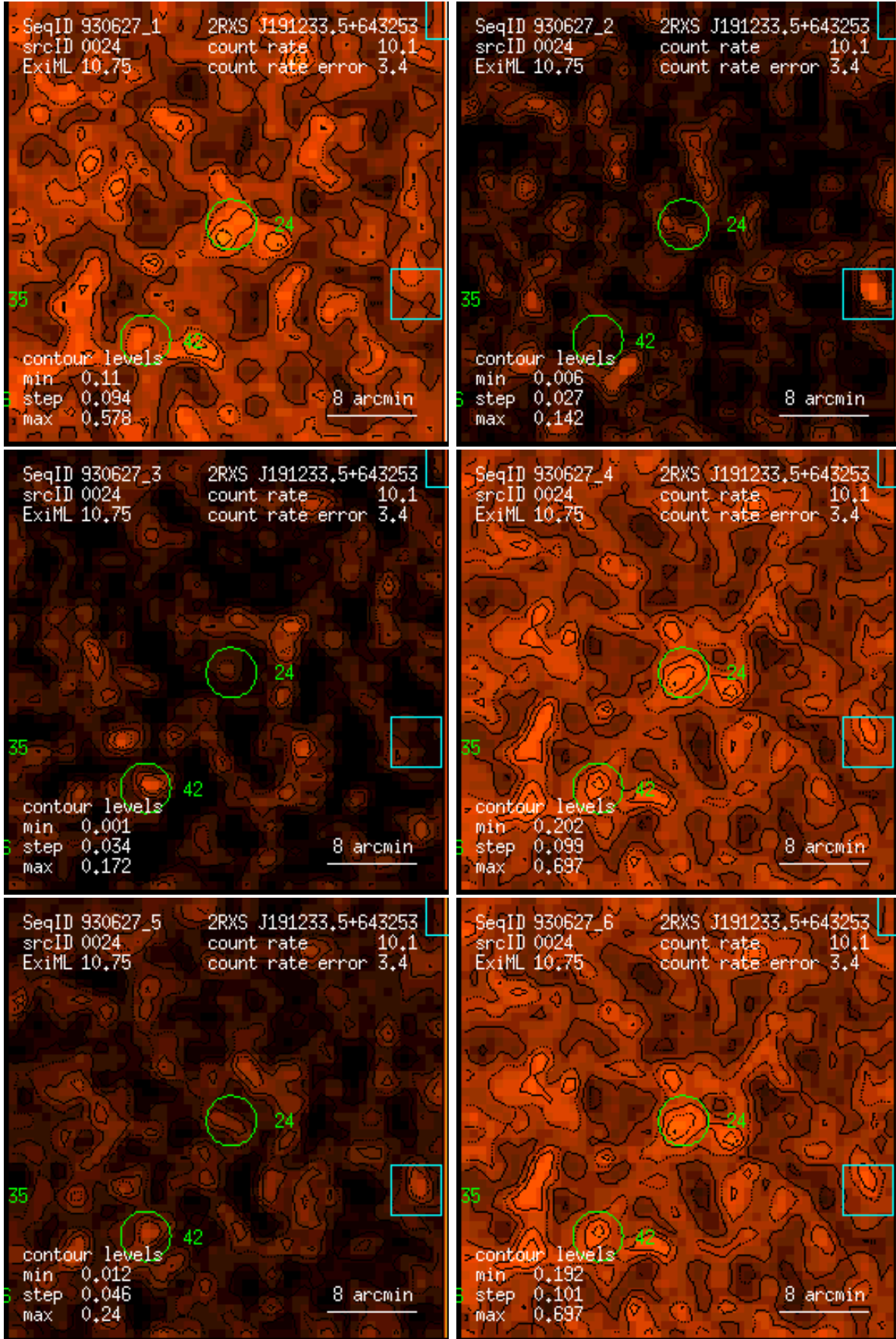
Figure 24: RASS 930627: detection 0024: band rate images, Gaussian filter: (1) PSPC channels 11 – 41, (2) 52 – 90, (3) 91 – 201, (4) 11 – 235, (5) 52 – 201, (6) 11 – 201. Broad band rates in counts/ks. Band rate contour levels in counts/ks/arcmin 2 .
