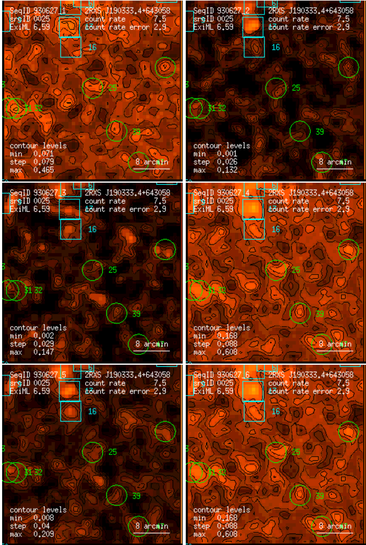
Figure 25: RASS 930627: detection 0025: band rate images, Gaussian filter: (1) PSPC channels 11 – 41, (2) 52 – 90, (3) 91 – 201, (4) 11 – 235, (5) 52 – 201, (6) 11 – 201. Broad band rates in counts/ks. Band rate contour levels in counts/ks/arcmin 2 .
