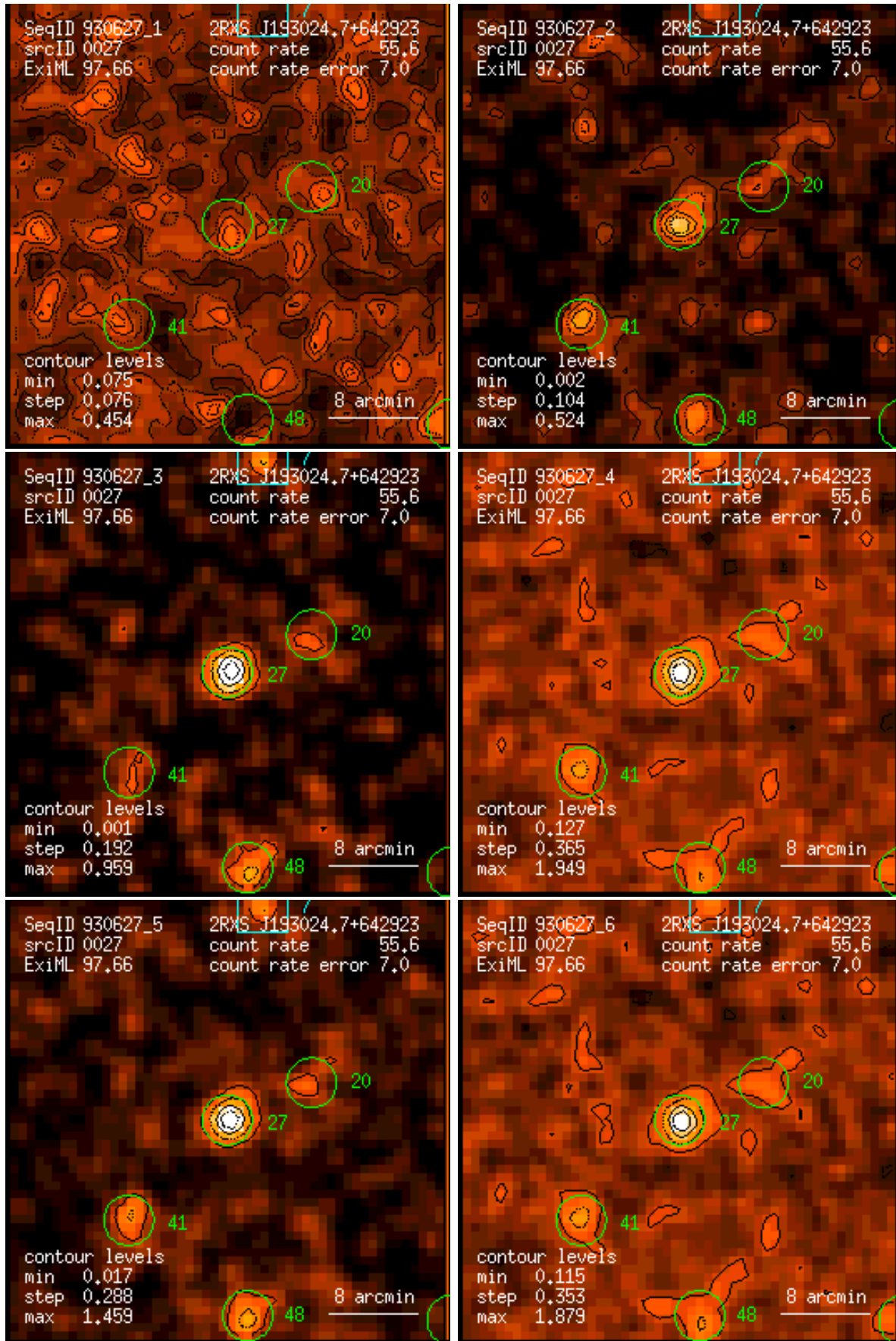
Figure 27: RASS 930627: detection 0027: band rate images, Gaussian filter: (1) PSPC channels 11 – 41, (2) 52 – 90, (3) 91 – 201, (4) 11 – 235, (5) 52 – 201, (6) 11 – 201. Broad band rates in counts/ks. Band rate contour levels in counts/ks/arcmin 2 .
