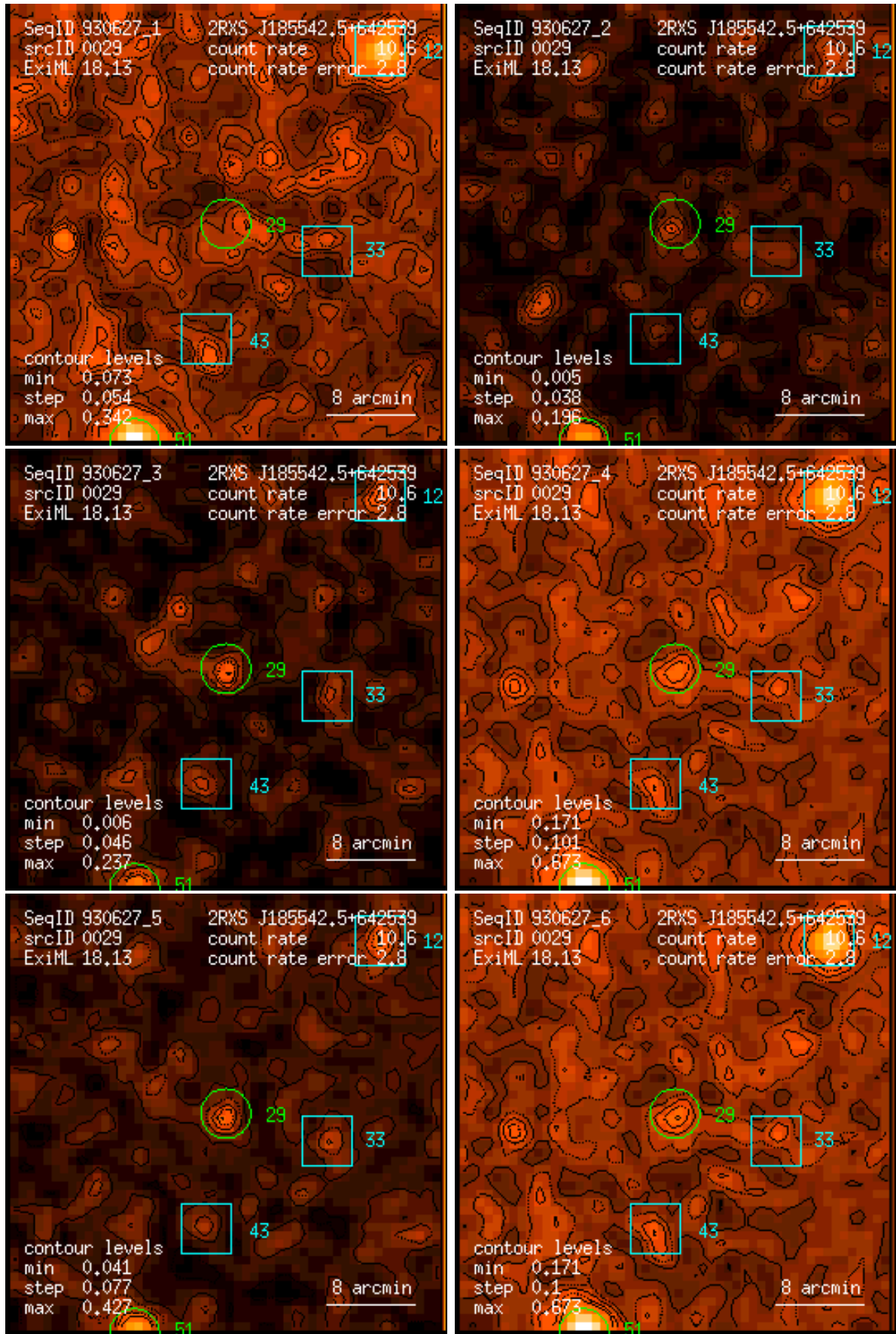
Figure 29: RASS 930627: detection 0029: band rate images, Gaussian filter: (1) PSPC channels 11 – 41, (2) 52 – 90, (3) 91 – 201, (4) 11 – 235, (5) 52 – 201, (6) 11 – 201. Broad band rates in counts/ks. Band rate contour levels in counts/ks/arcmin 2 .
