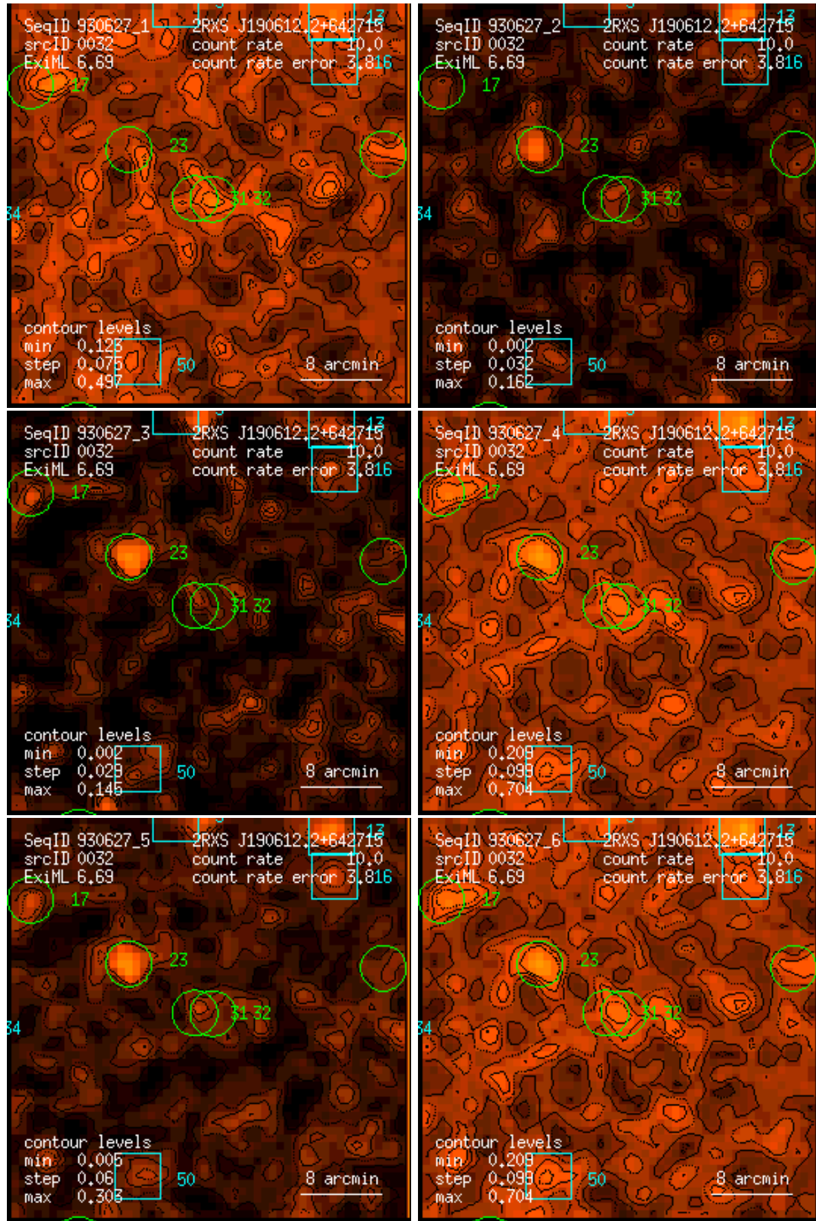
Figure 32: RASS 930627: detection 0032: band rate images, Gaussian filter: (1) PSPC channels 11 – 41, (2) 52 – 90, (3) 91 – 201, (4) 11 – 235, (5) 52 – 201, (6) 11 – 201. Broad band rates in counts/ks. Band rate contour levels in counts/ks/arcmin 2 .
