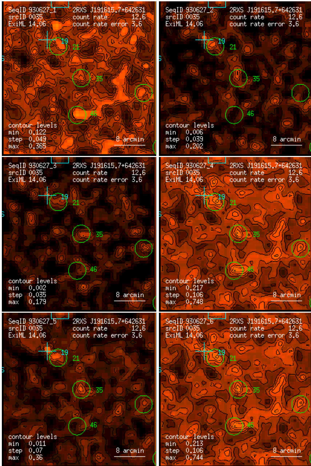
Figure 35: RASS 930627: detection 0035: band rate images, Gaussian filter: (1) PSPC channels 11 – 41, (2) 52 – 90, (3) 91 – 201, (4) 11 – 235, (5) 52 – 201, (6) 11 – 201. Broad band rates in counts/ks. Band rate contour levels in counts/ks/arcmin 2 .
