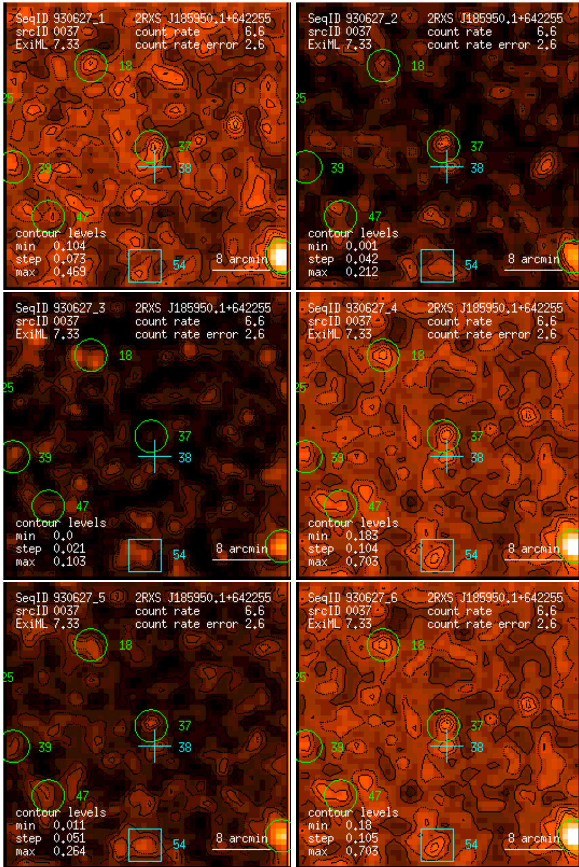
Figure 37: RASS 930627: detection 0037: band rate images, Gaussian filter: (1) PSPC channels 11 – 41, (2) 52 – 90, (3) 91 – 201, (4) 11 – 235, (5) 52 – 201, (6) 11 – 201. Broad band rates in counts/ks. Band rate contour levels in counts/ks/arcmin 2 .
