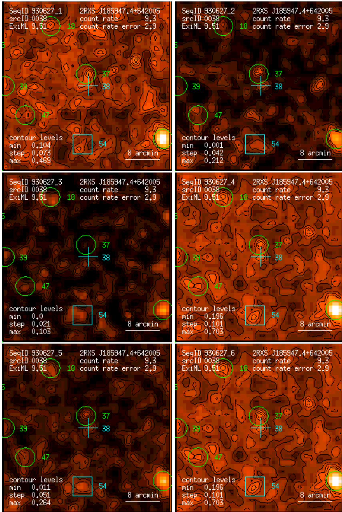
Figure 38: RASS 930627: detection 0038: band rate images, Gaussian filter: (1) PSPC channels 11 – 41, (2) 52 – 90, (3) 91 – 201, (4) 11 – 235, (5) 52 – 201, (6) 11 – 201. Broad band rates in counts/ks. Band rate contour levels in counts/ks/arcmin 2 .
